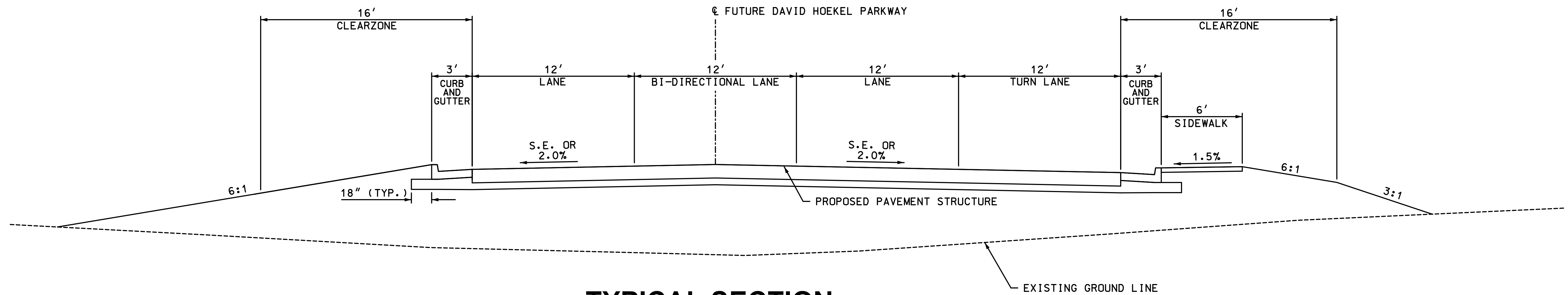
TYPICAL SECTION FUTURE DAVID HOEKEL PARKWAY
