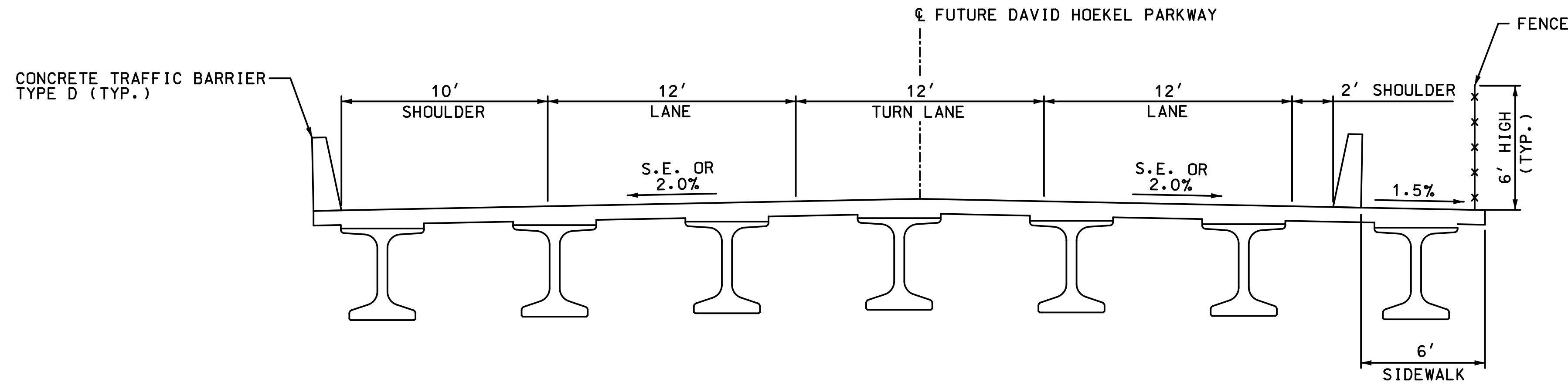
TYPICAL SECTION FUTURE DAVID HOEKEL PARKWAY BRIDGE OVER U.S. ROUTE 61
