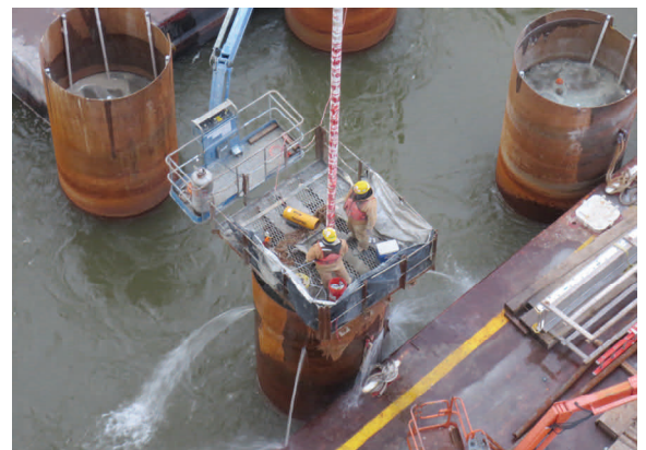
Crews pouring concrete into the shafts for the new Boone Bridge.
