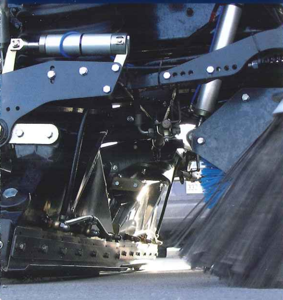
BELOW Optional full-width nozzle option between the axles.
