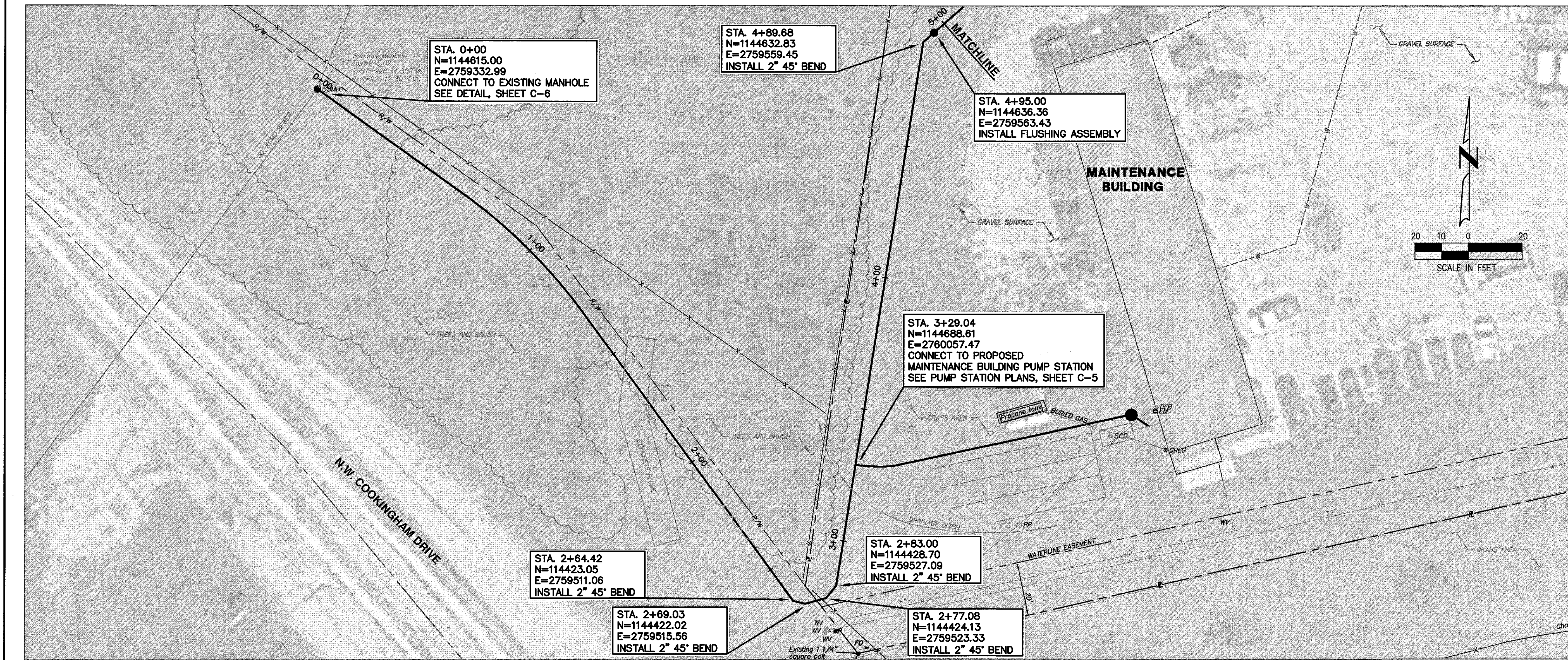
PRESSURE SEWER PLAN
