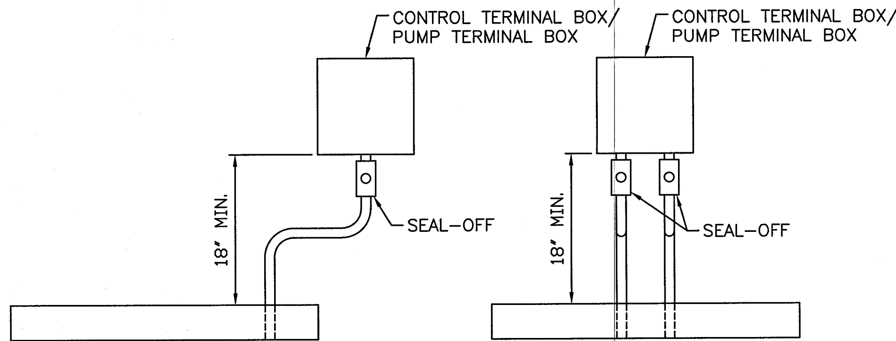
SIDE VIEW
