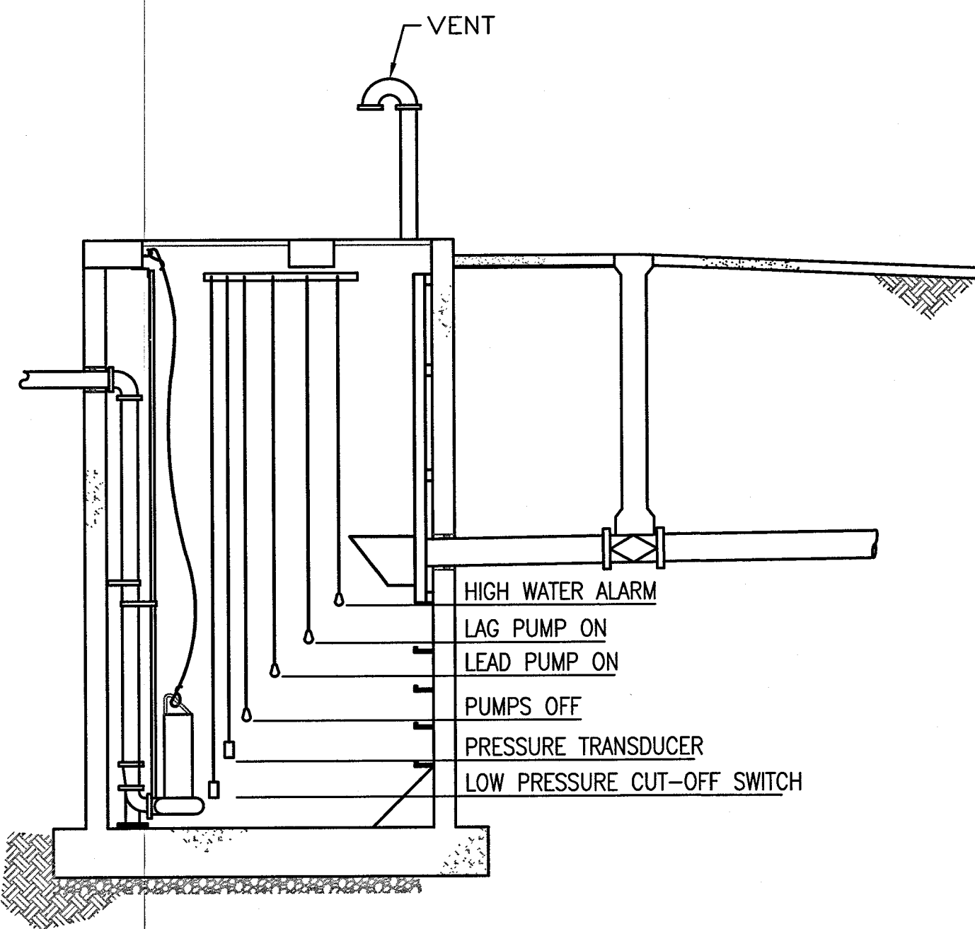
PUMP STATION SECTION
