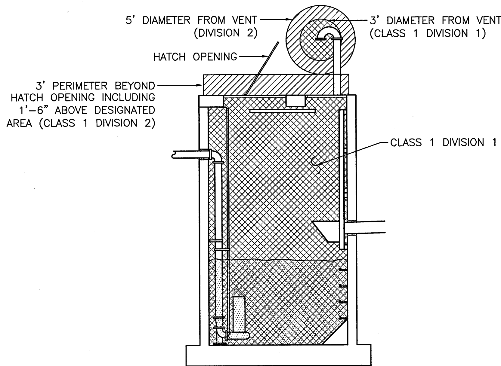
WET WELL AREA CLASSIFICATION
