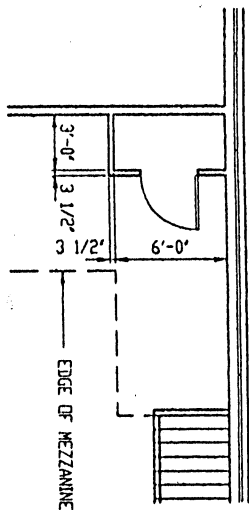
COMMUNICATION CLOSET (BUILD ON MEZZANINE) 3/32" = 1'-0"
