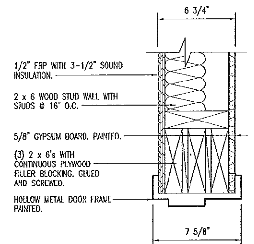
D 15 JAMB SIMILAR DOOR HEAD SCALE: 1-1/2" = 1'-0"
