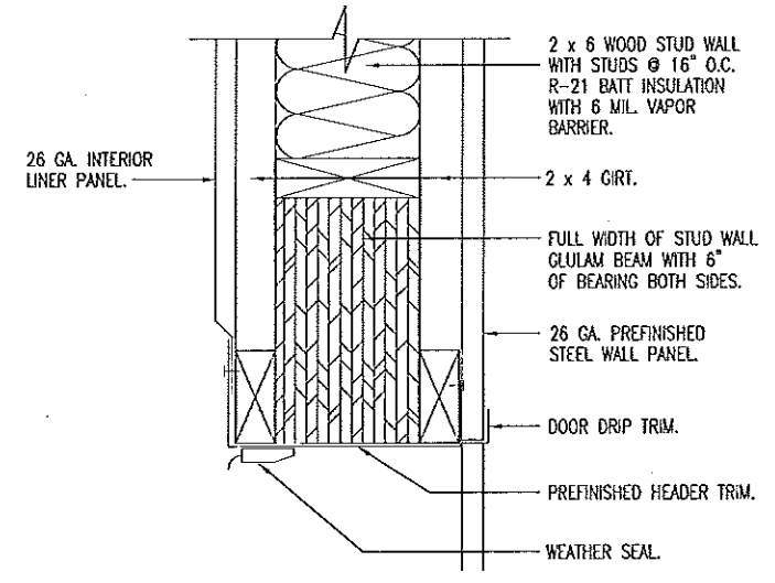
B 14 GARAGE DOOR HEAD SCALE: 1-1/2" = 1'-0"
