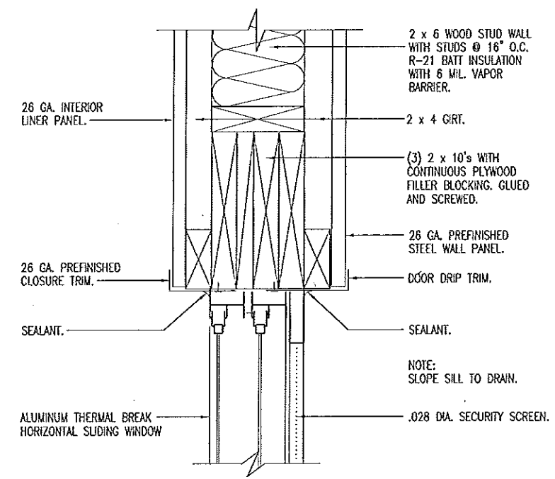
F 14 JAMB & SILL SIMILAR WINDOW HEAD SCALE: 1-1/2" = 1'-0"
