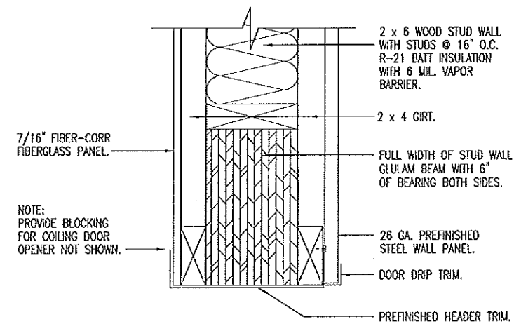
B 15 COILING GARAGE DOOR HEAD SCALE: 1-1/2" = 1'-0"
