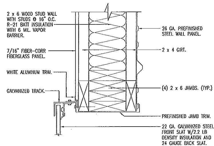
A 15 COILING GARAGE DOOR JAMB SCALE: 1-1/2" = 1'-0"
