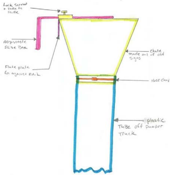
Concrete Wonder Chute side view
