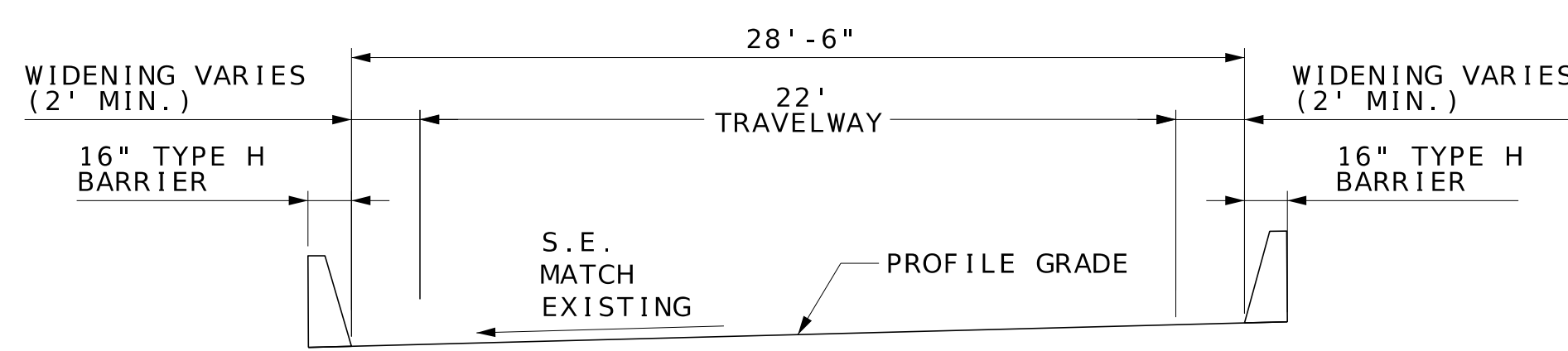
TYPICAL SECTION ROUTE H STA. 355+60.50 - STA. 356+82.45 (PROPOSED BRIDGE) NOT TO SCALE
