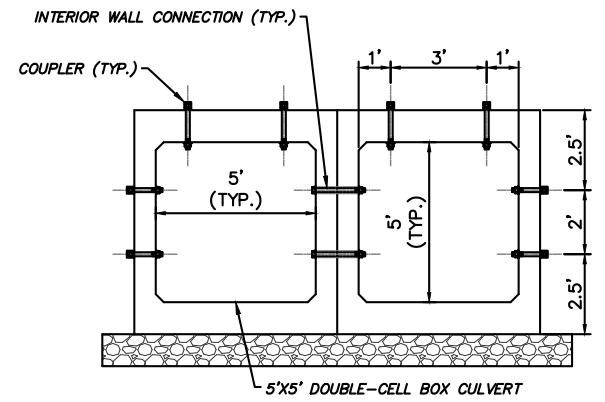
DOUBLE-CELL CONNECTION DETAILS
