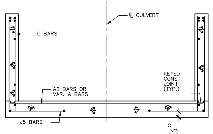
UPSTREAM AND DOWNSTREAM WINGS REINFORCEMENT
