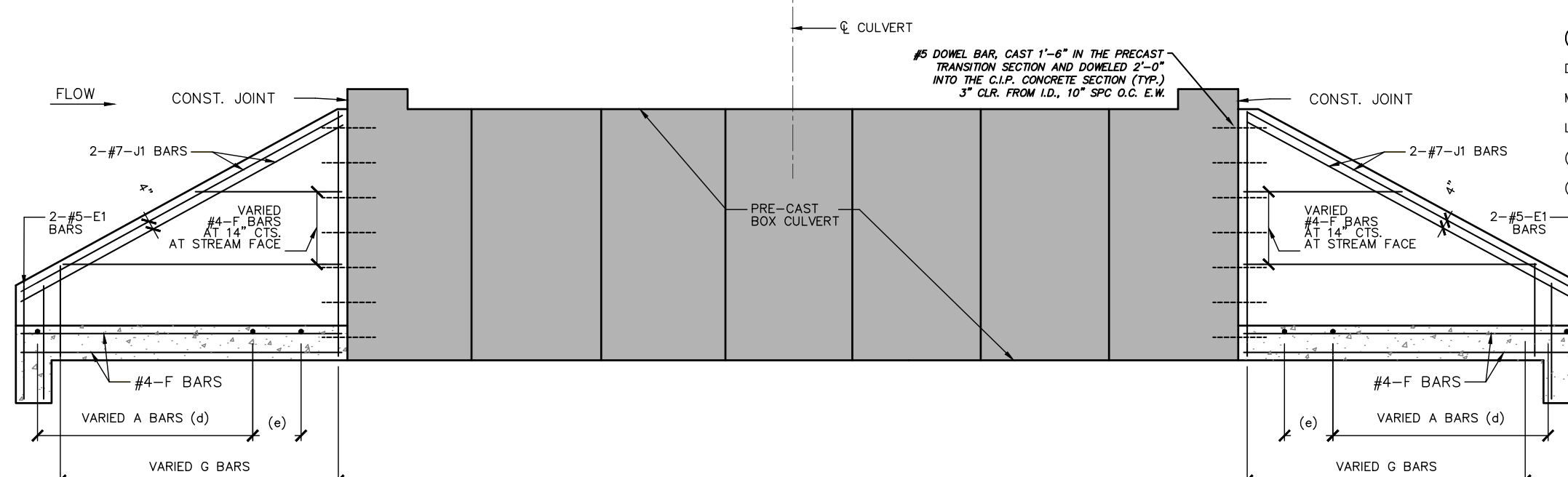
ELEVATION OF PRECAST BOX WITH CAST IN PLACE WINGWALLS
