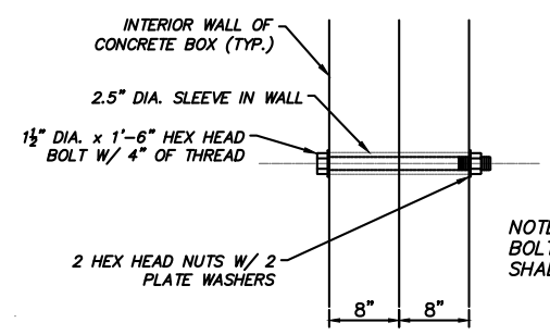
INTERIOR SIDEWALL CONNECTION DETAIL
