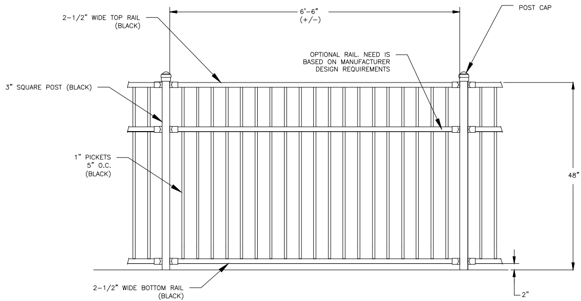
FENCE SECTION ELEVATION
