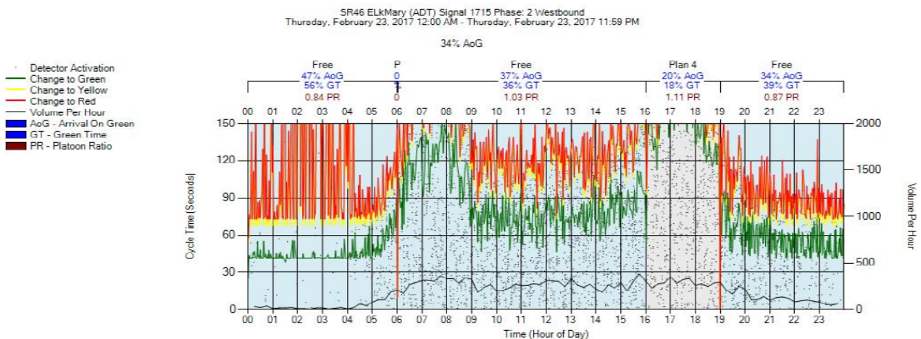
Figure 1 – Purdue Coordination Diagram
