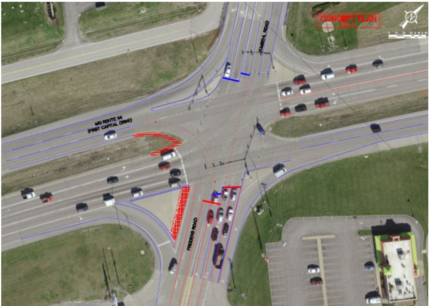
Concept Plan 1 – Zumbahl Road/Friedens Road Intersection
