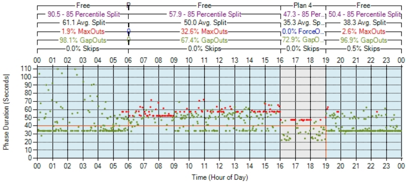
Figure 2 – Split Monitoring Diagram
