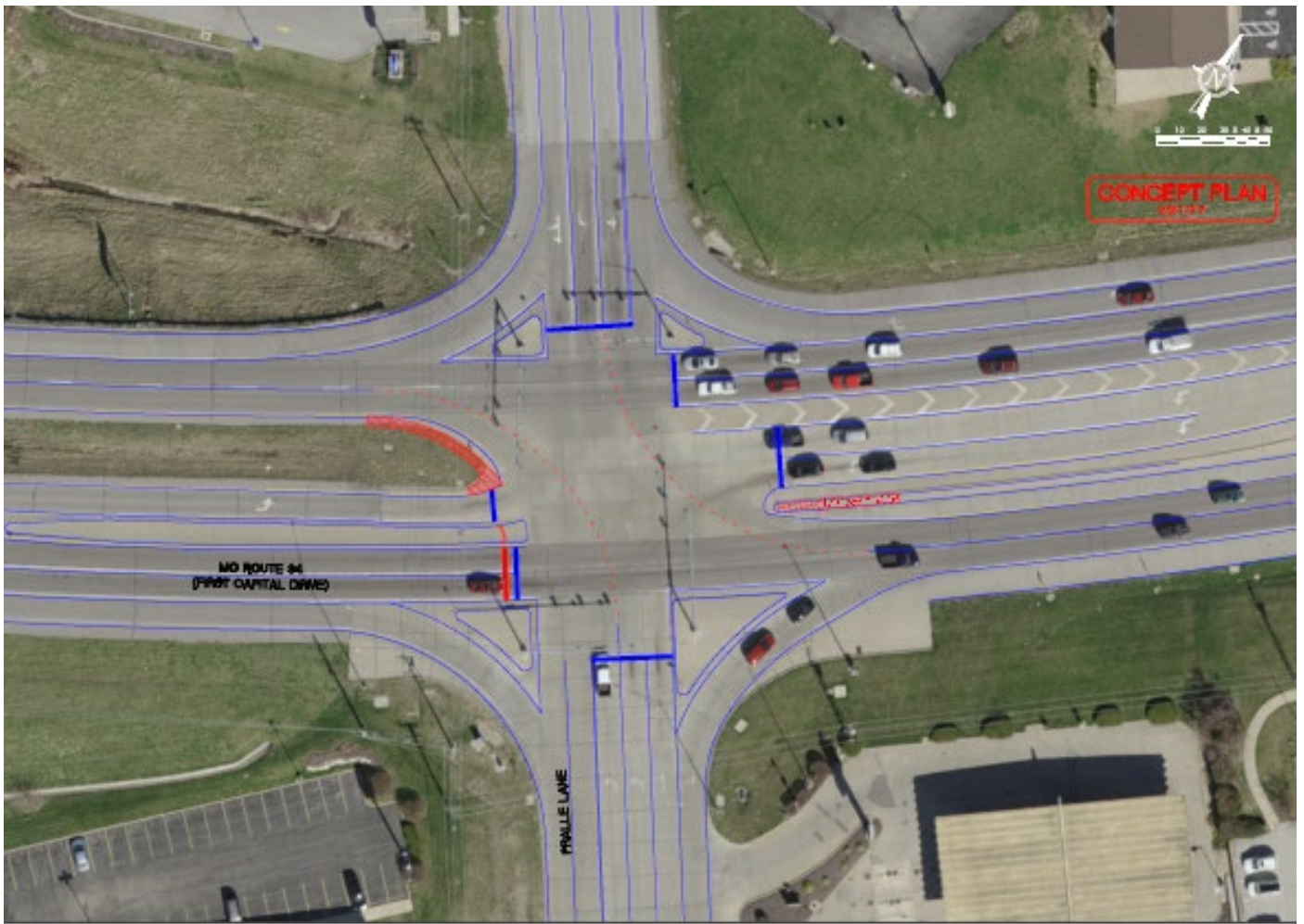
Concept Plan 2 – Pralle Lane Intersection
