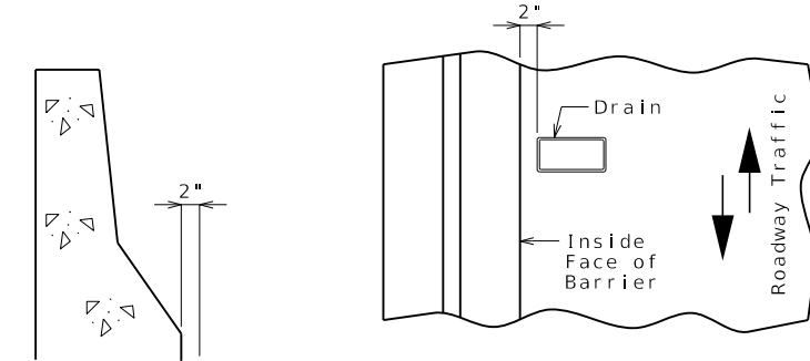
PART PLAN OF SLAB AT DRAIN
