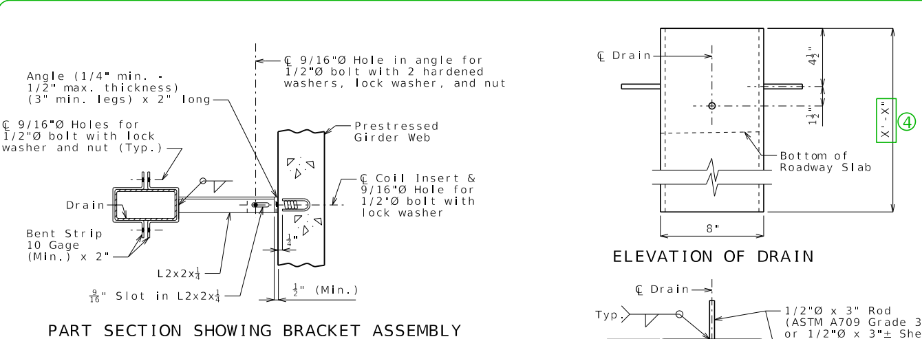
PART SECTION SHOWING BRACKET ASSEMBLY
