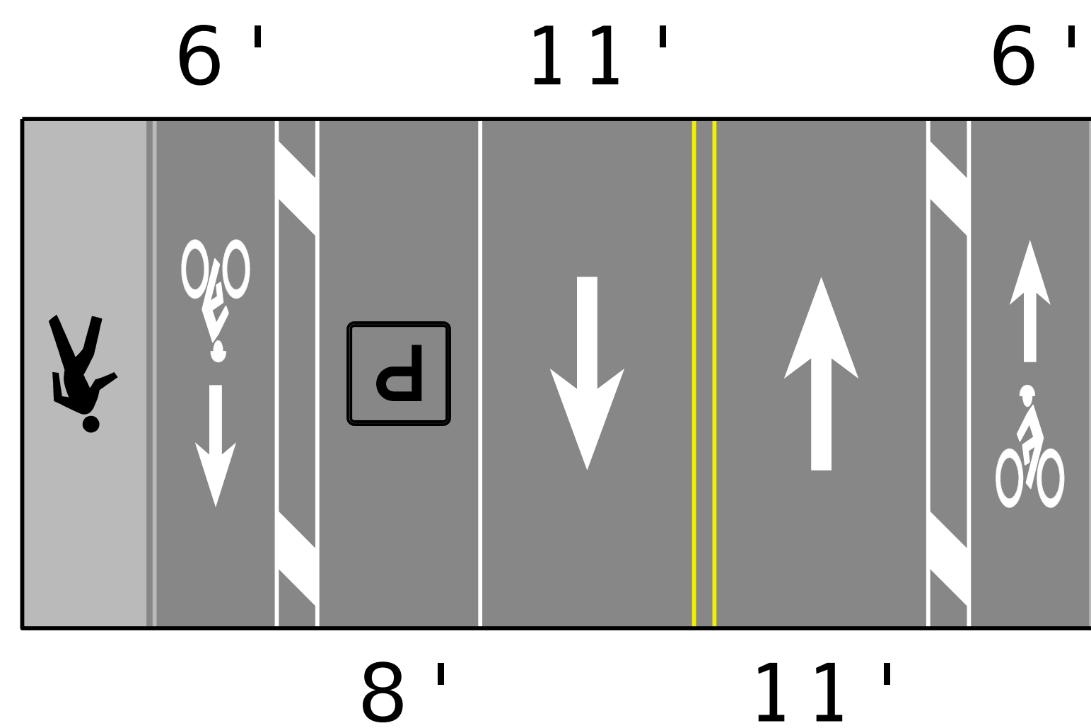
OPTION 1 (w/2' BIKE BUFFER)
