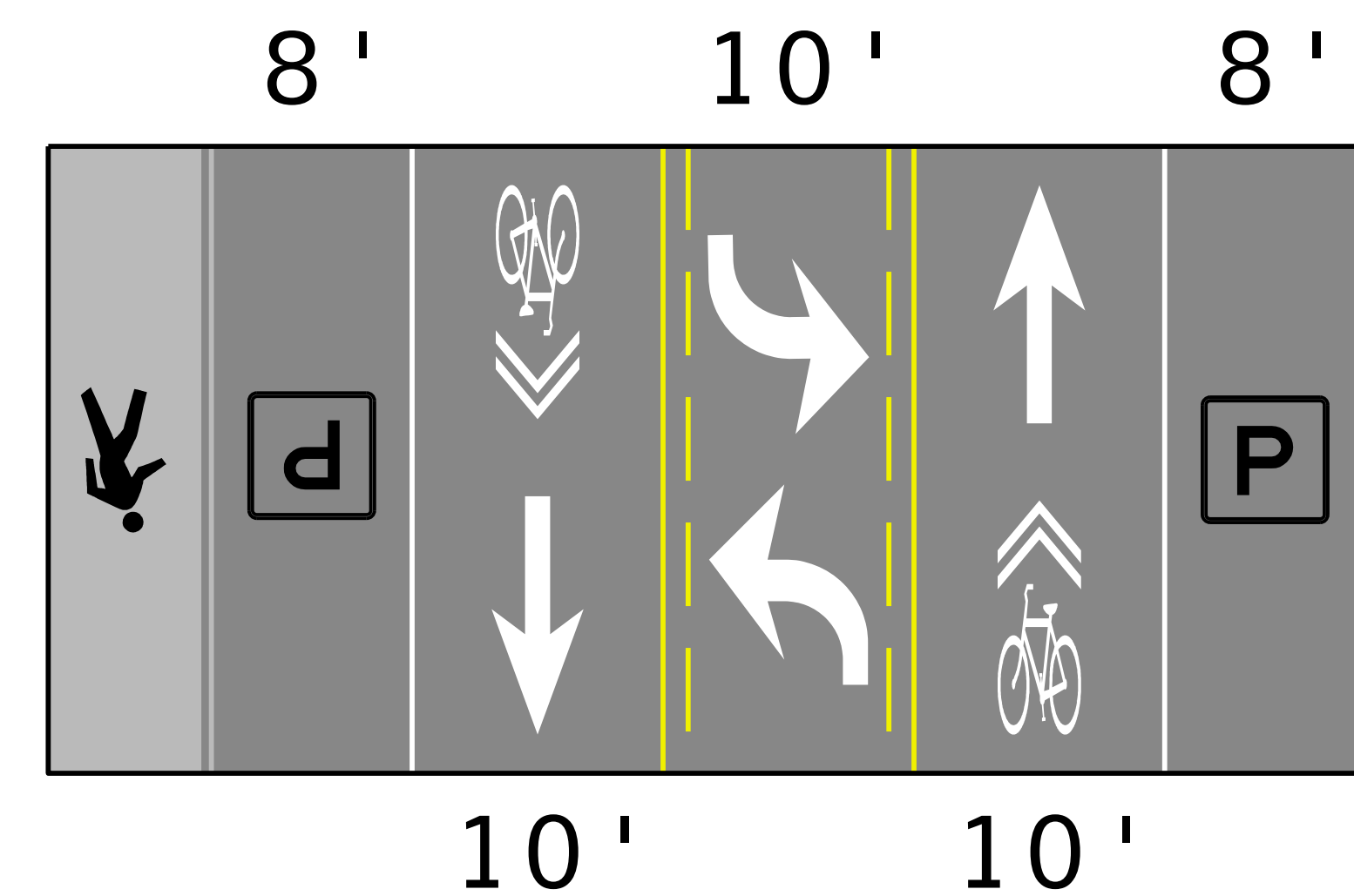
OPTION 3 (TWO-WAY LEFT TURN LANE w/PARKING LANES)
