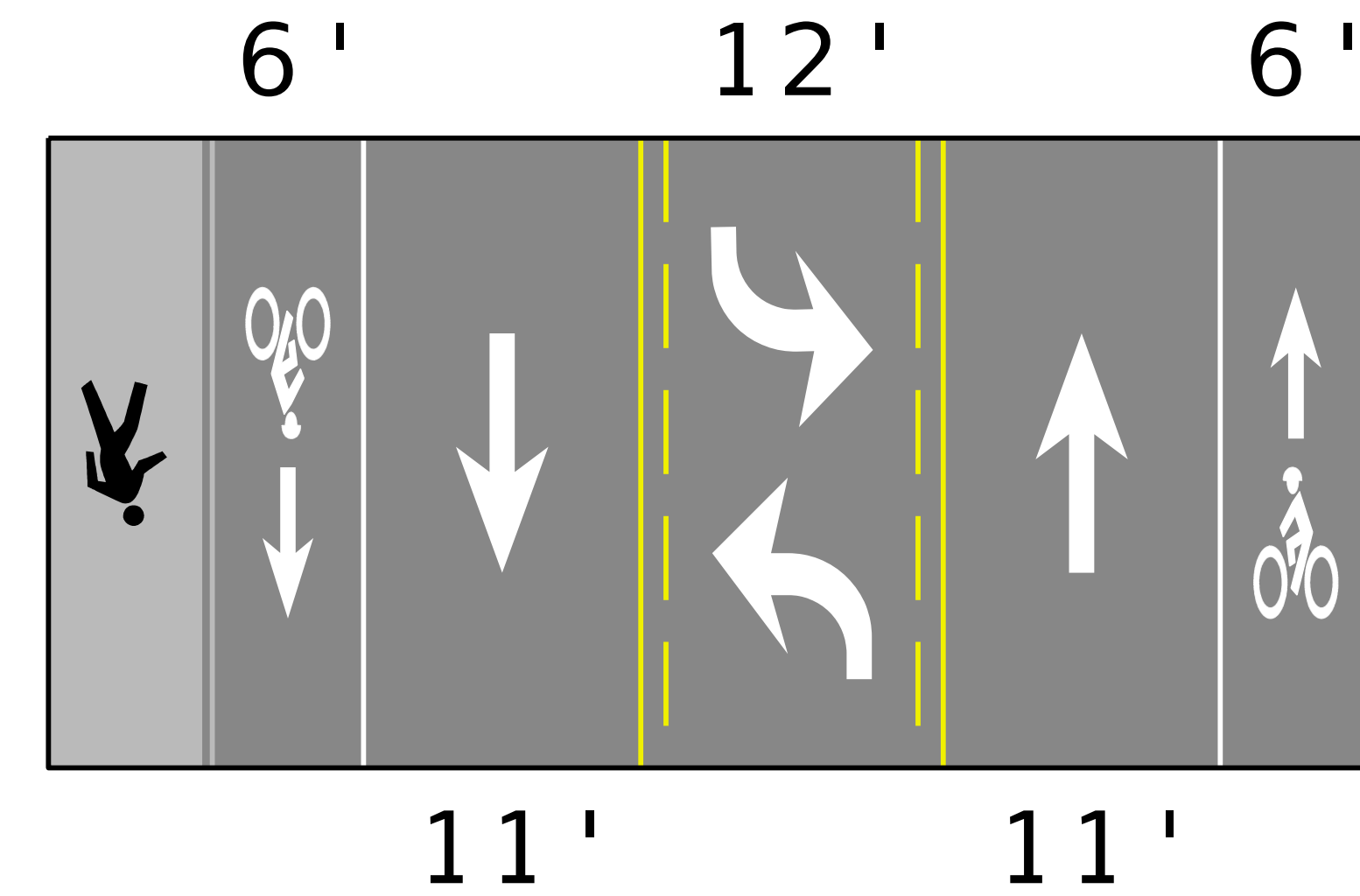
OPTION 2 (TWO-WAY LEFT TURN LANE w/BIKE LANES)
