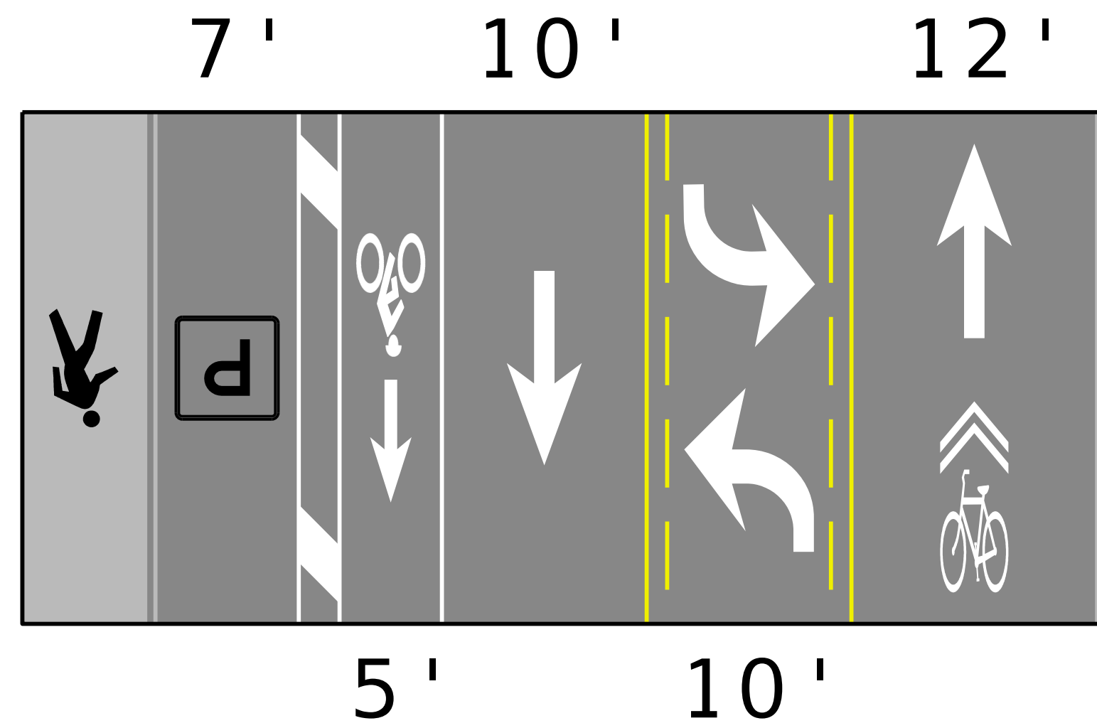
EXISTING STRIPING (w/2' BIKE BUFFER)
