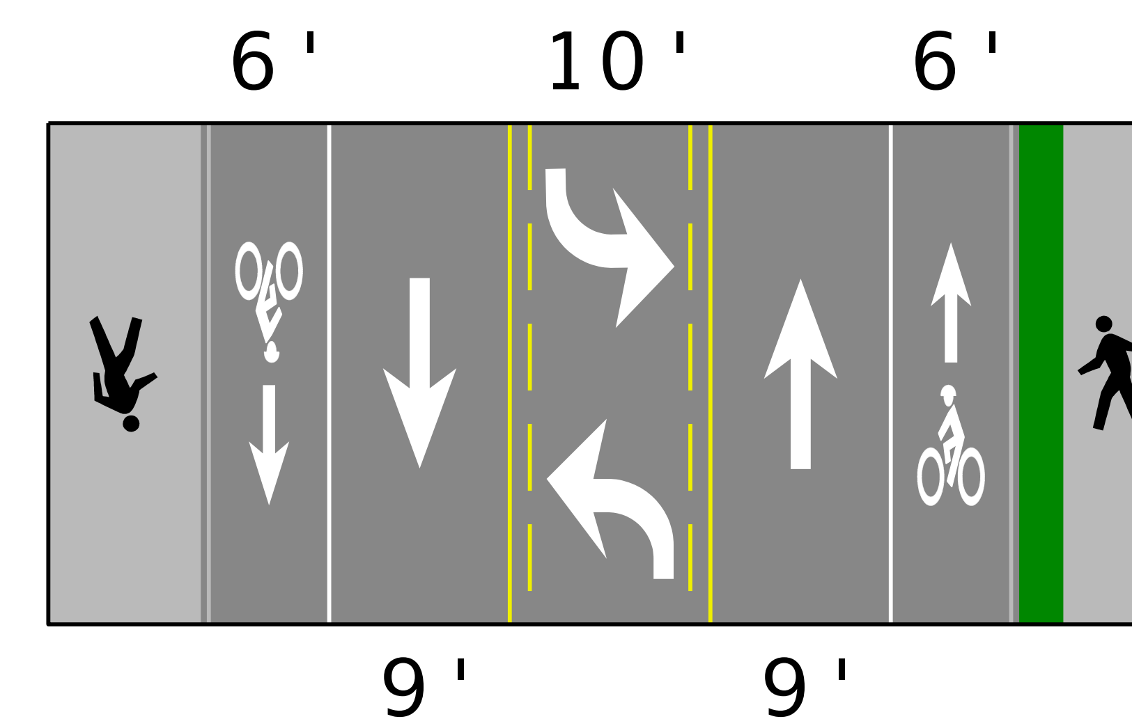
OPTION 3 (TWO-WAY LEFT TURN LANE w/BIKE LANES)
