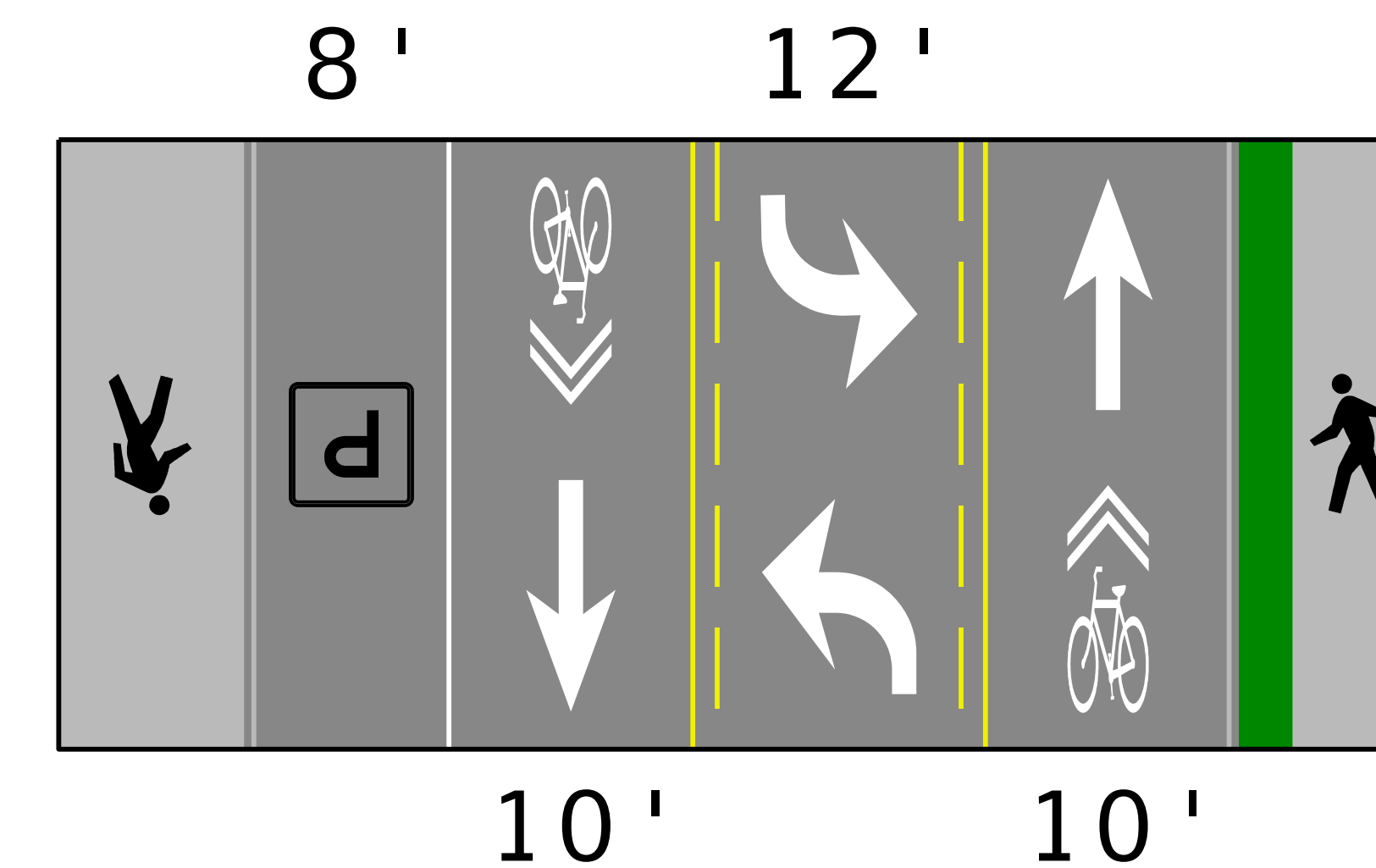
OPTION 2 (TWO-WAY LEFT TURN LANE)
