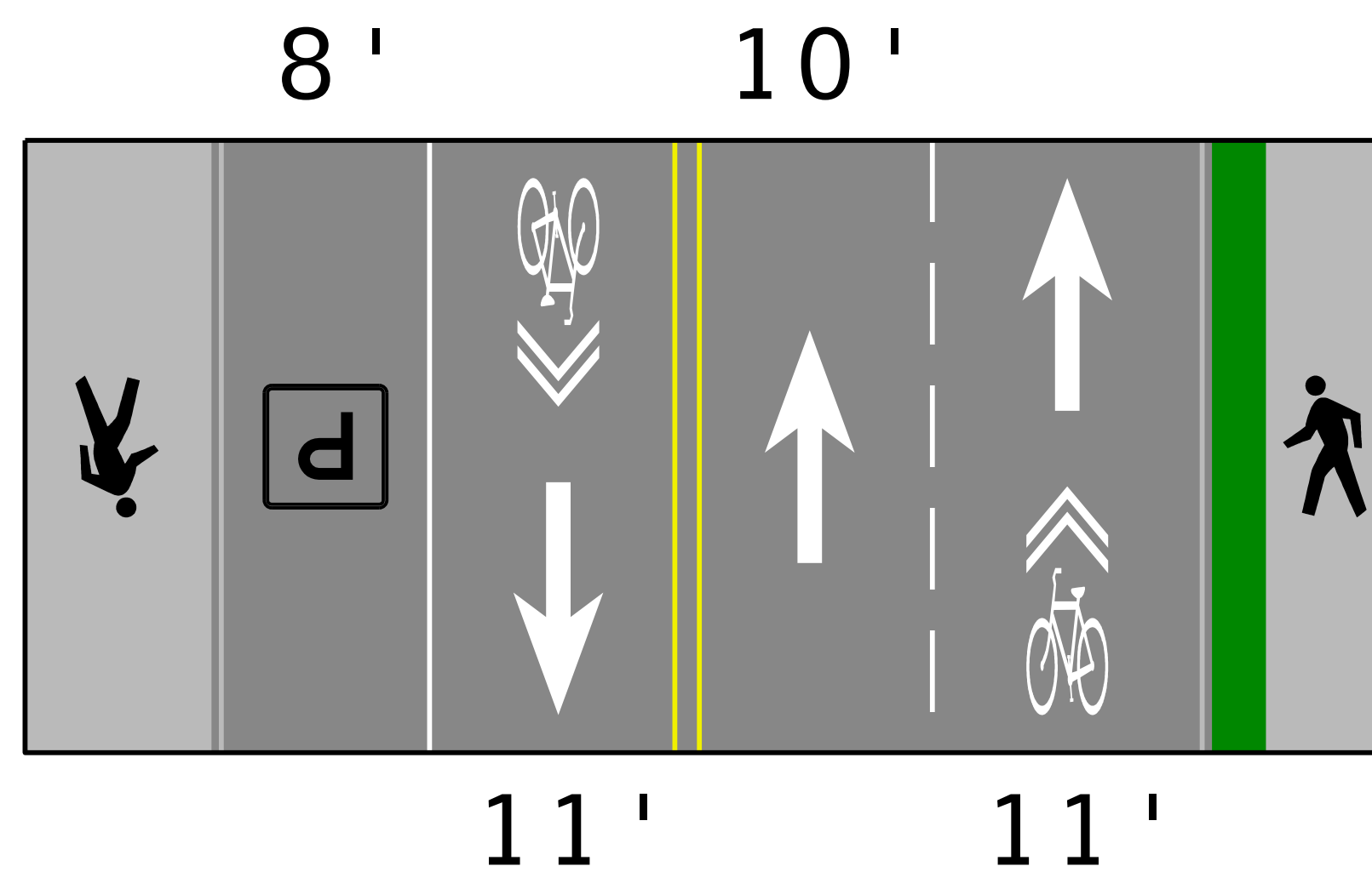
EXISTING STRIPING
