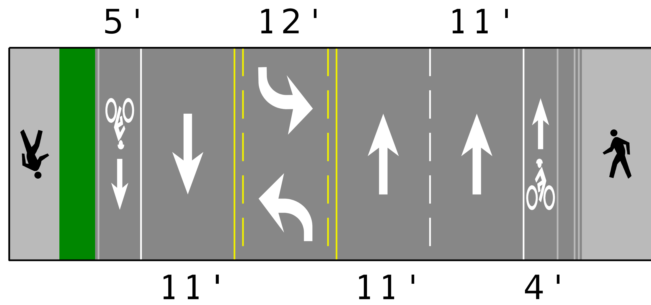
EXISTING STRIPING
