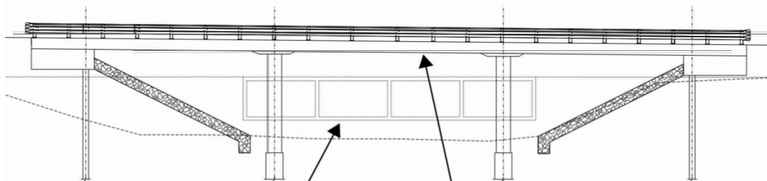
(33'-40'-33') CONTINUOUS CONCRETE SOLID SLAB BRIDGE
