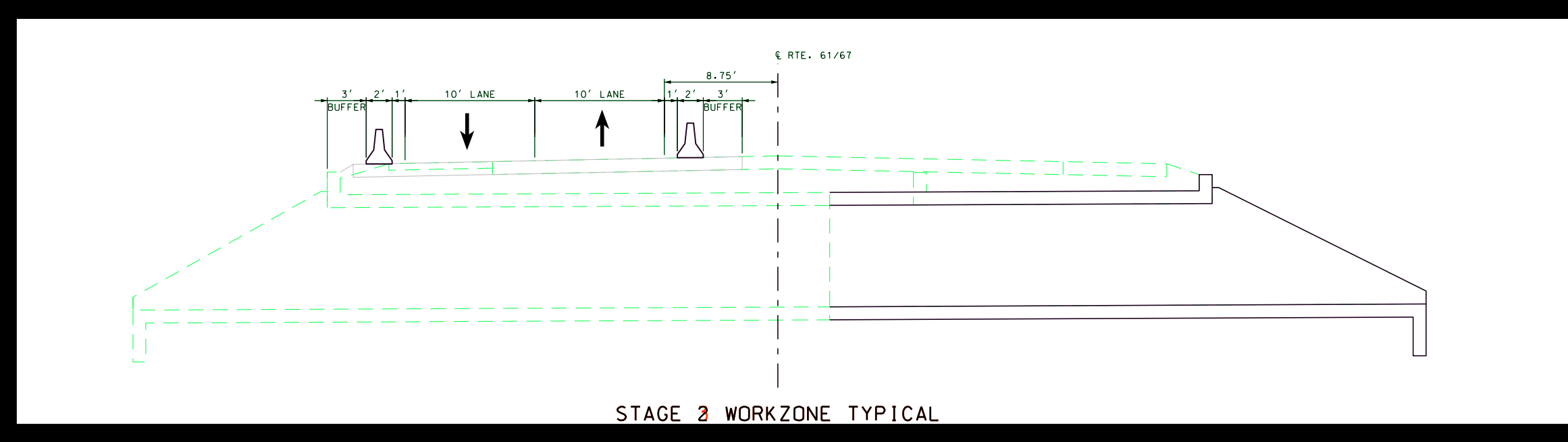
CULVERT 1 AND 2 CONSTRUCTION STAGE 2
