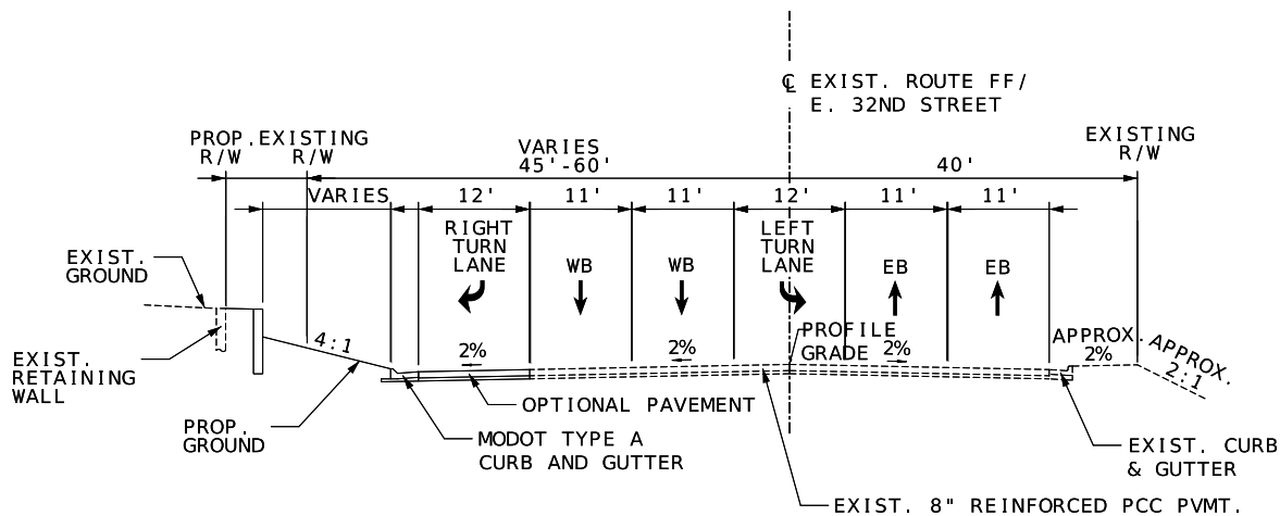
PROPOSED RTE. FF/ E. 32ND ST. STA. 35+13.88 TO STA. 39+28.96
