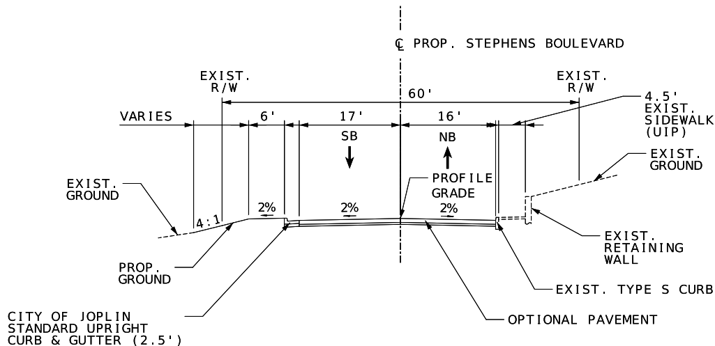
PROP. STEPHENS BOULEVARD STA. 11+14.83 TO STA. 12+52.32
