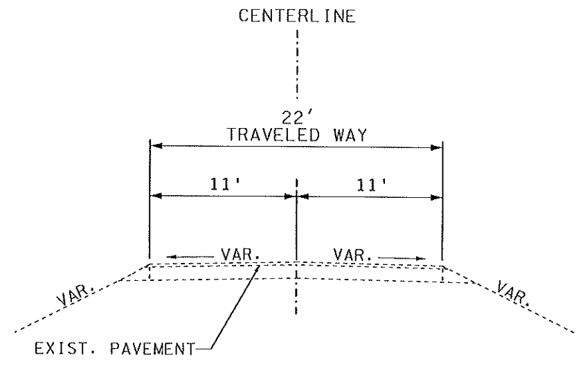
EXISTING TYPICAL SECTION ROUTE 89 STA. 649+98.17 TO STA. 652+26.00 STA. 652+61.00 TO STA. 653+55.57
