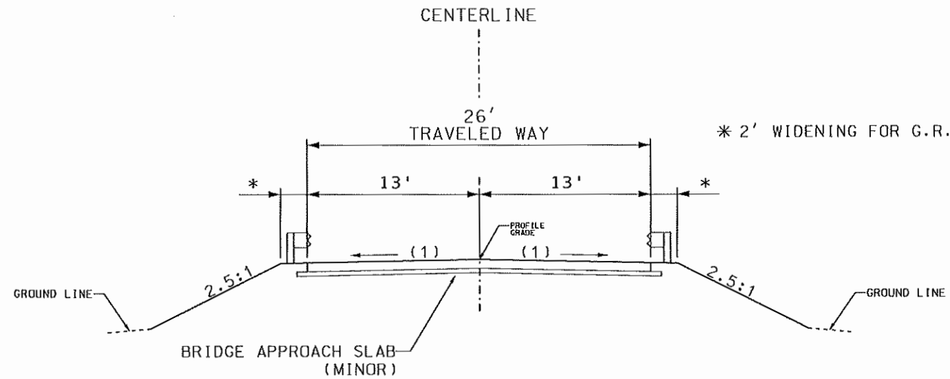
BRIDGE APPROACH SLAB MINOR ROUTE 20' EACH END ROUTE 89 STA. 651+82.11 TO STA. 652+02.11 STA. 652+95.61 TO STA. 653+15.61
