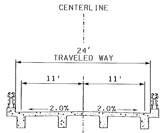
EXISTING BRIDGE TYPICAL SECTION ROUTE 89 STA. 652+26.00 TO STA. 652+61.00
