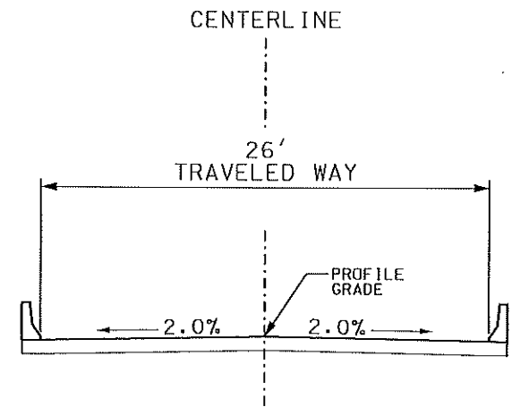
PROPOSED BRIDGE TYPICAL SECTION ROUTE 89 STA. 652+02.11 TO STA. 652+95.61
