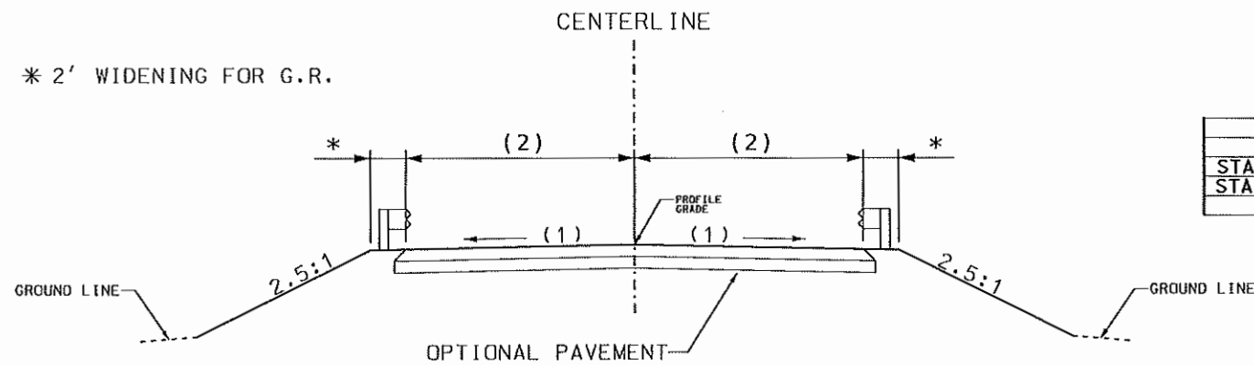
PROPOSED TYPICAL SECTION ROUTE 89 STA. 649+98.17 TO STA. 651+82.11 STA. 653+15.61 TO STA. 653+55.57
