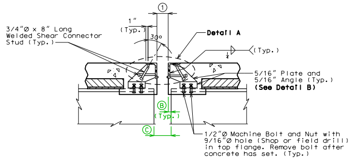
PART SECTION A-A
