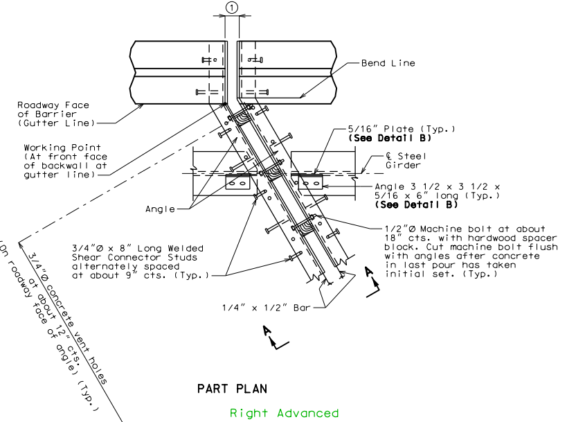
PART PLAN
