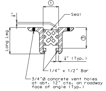
SECTION THRU DEVICE
