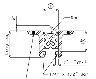
SECTION THRU DEVICE
