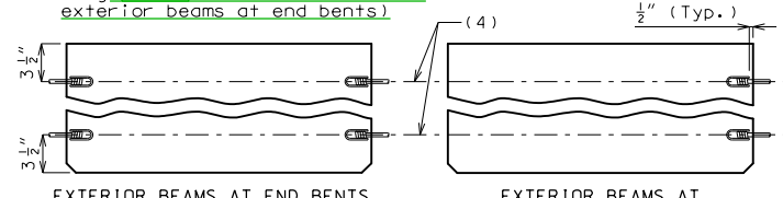
COIL TIES
