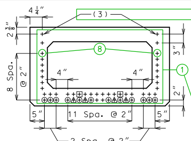
STRAND ARRANGEMENT
