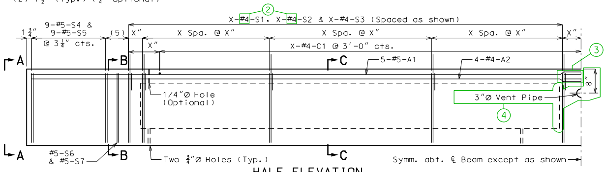
HALF ELEVATION
