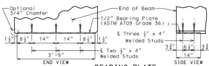
BEARING PLATE
