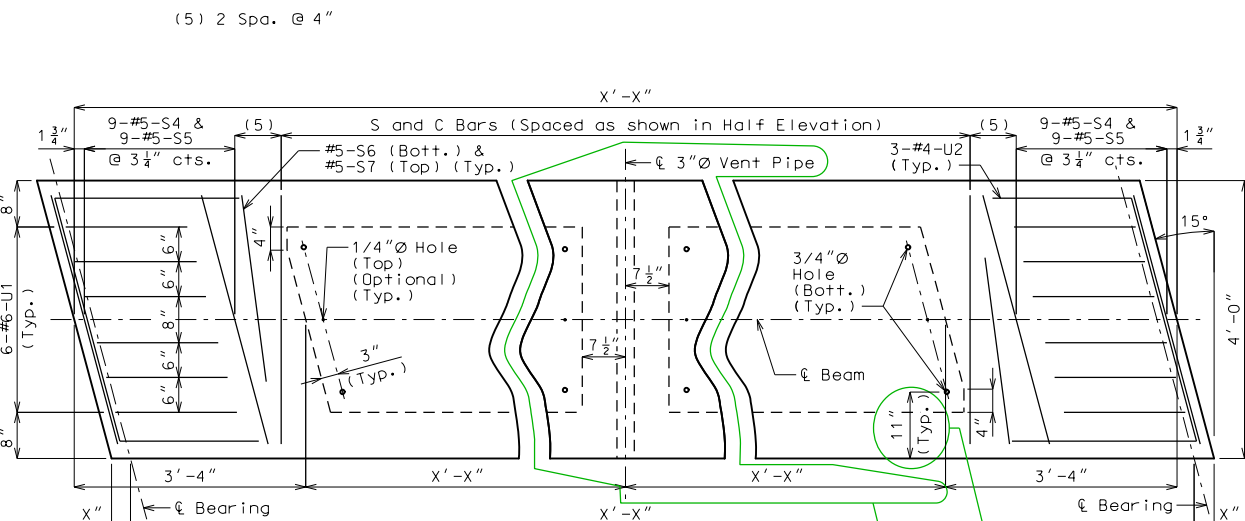
PART PLAN
