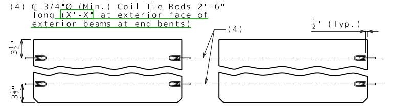
COIL TIES
