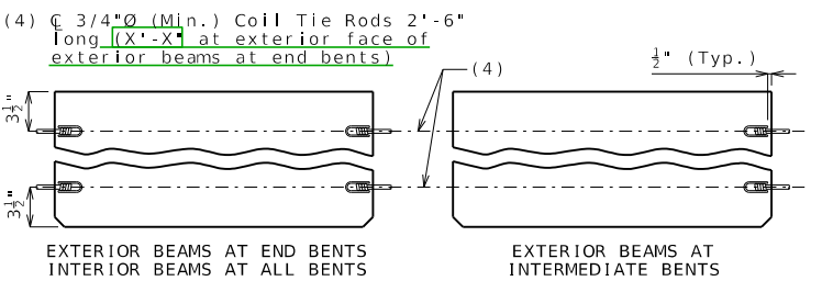
COIL TIES
