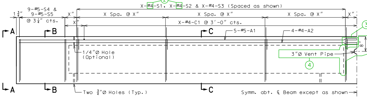
HALF ELEVATION
