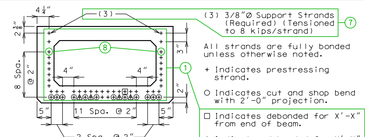
STRAND ARRANGEMENT
