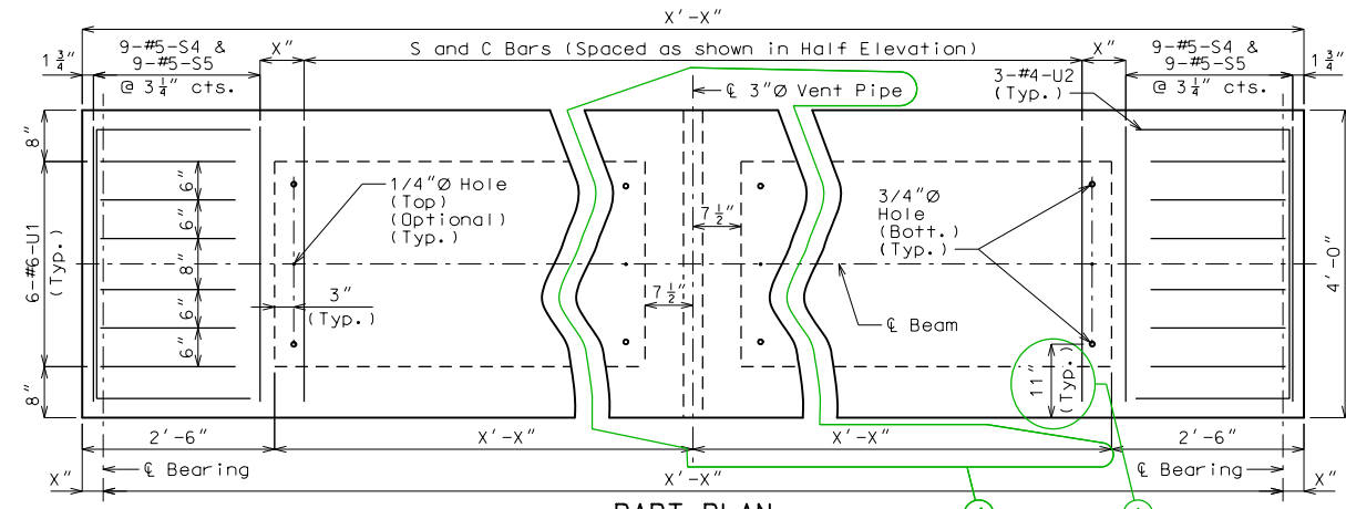
PART PLAN
