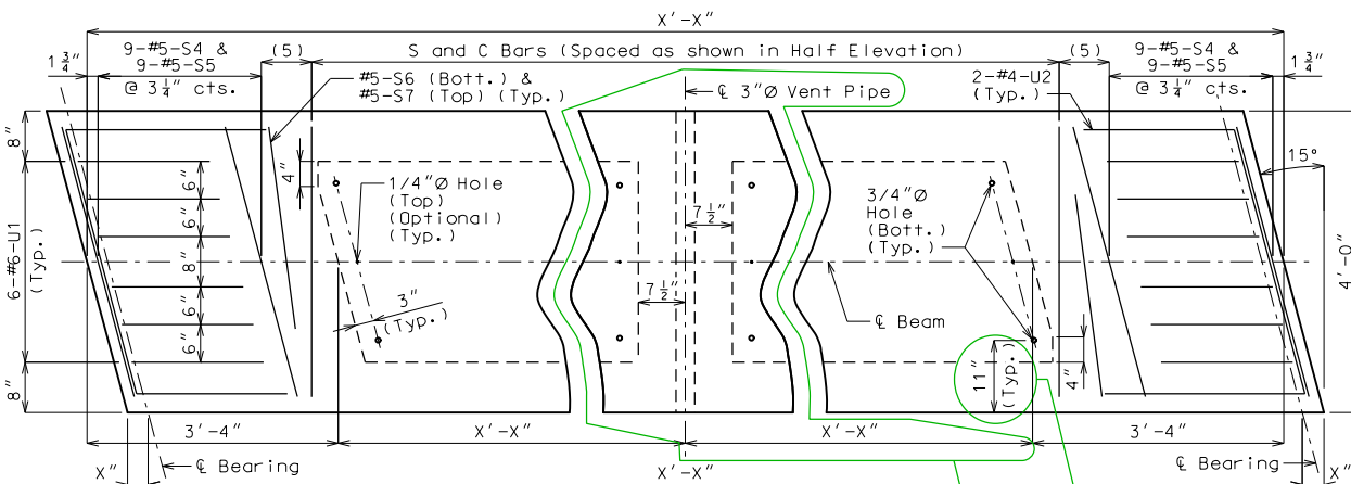
PART PLAN
