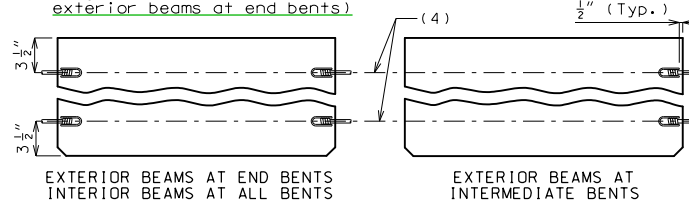
COIL TIES
