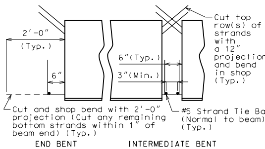
STRANDS AT BEAM ENDS
