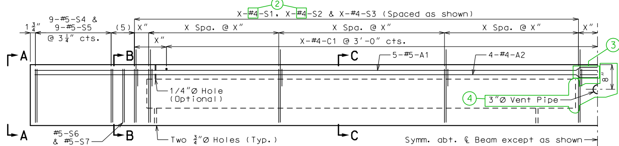
HALF ELEVATION
