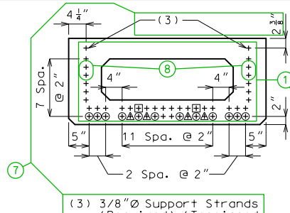
STRAND ARRANGEMENT
