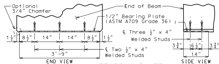
BEARING PLATE
