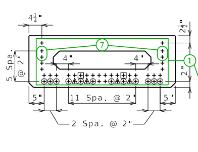
STRAND ARRANGEMENT
