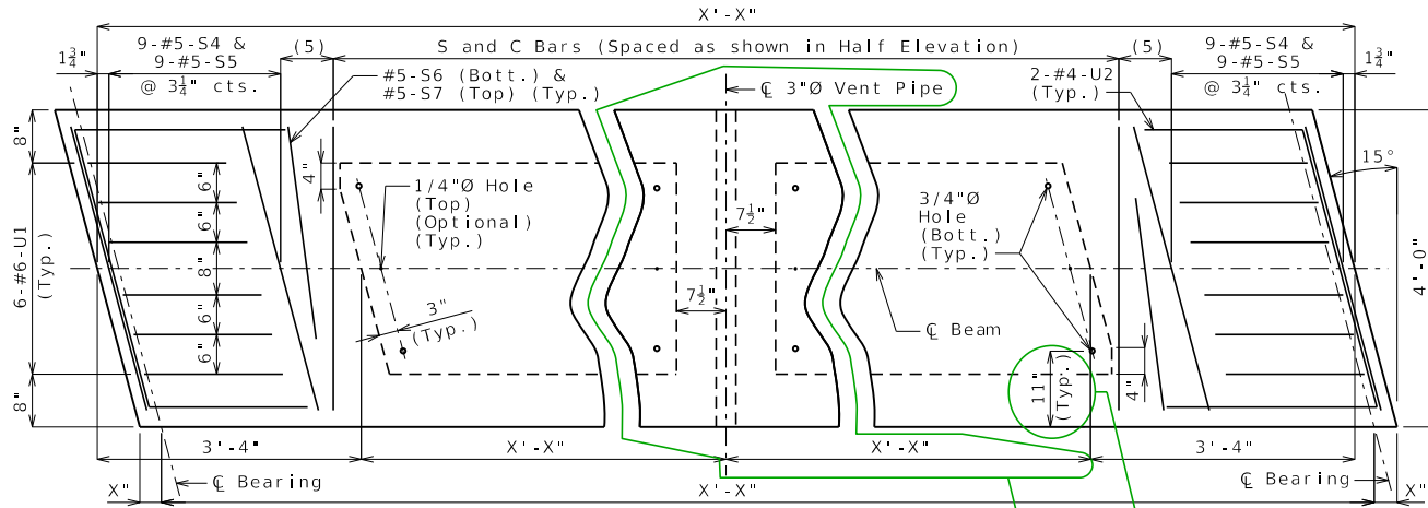
PART PLAN
