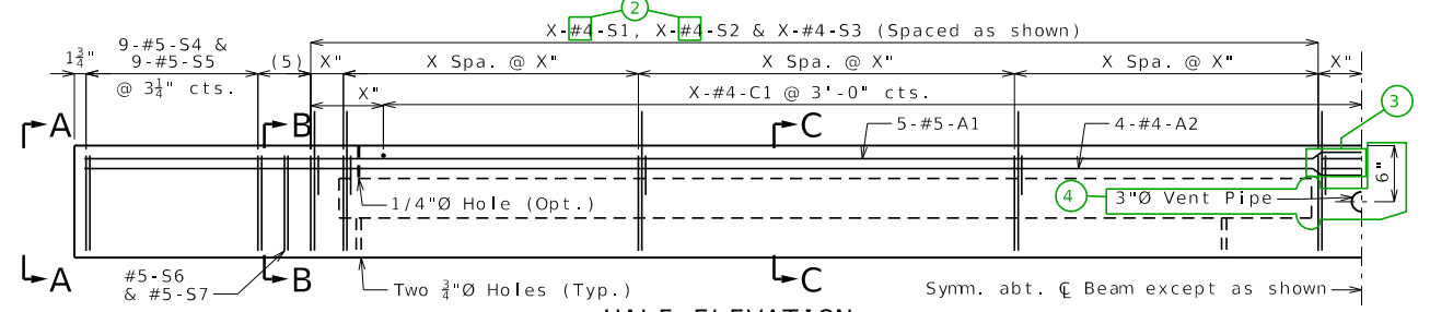
HALF ELEVATION
