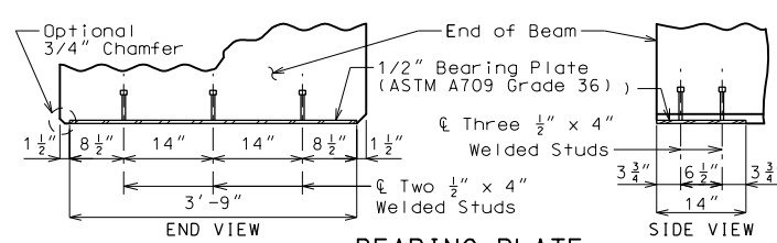
BEARING PLATE
