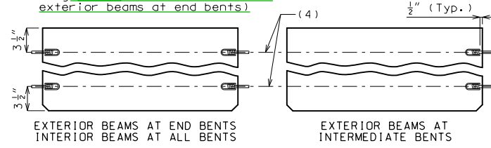
COIL TIES
