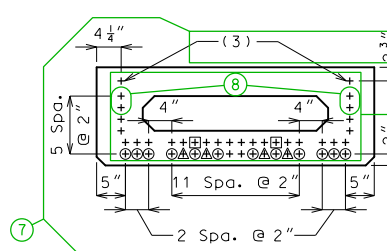
STRAND ARRANGEMENT
