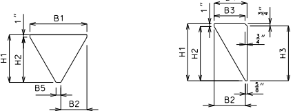
T1 PLATE DETAILS T2 PLATE DETAILS (2 REQUIRED)
