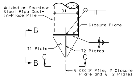
CRUCIFORM PILE POINT
