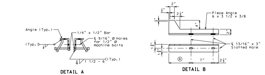
DETAIL A
