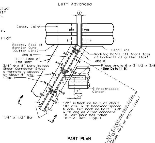
PART PLAN
