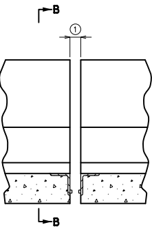
PART ELEVATION OF BARRIER CURB
