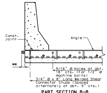
PART SECTION B-B ** Extend preformed compression seal 3" past the edge of slab (Typ.)
