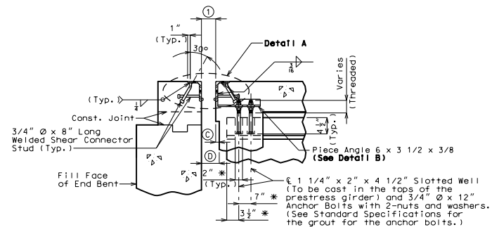
PART SECTION A-A * Dimension along G Girder
