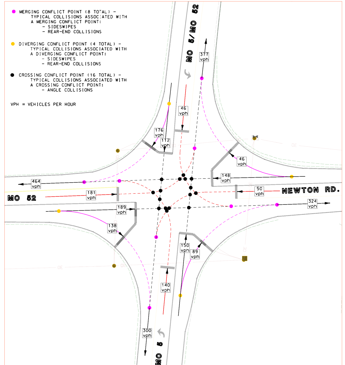
FOUR-LEGGED INTERSECTION - 28 CONFLICT POINTS
