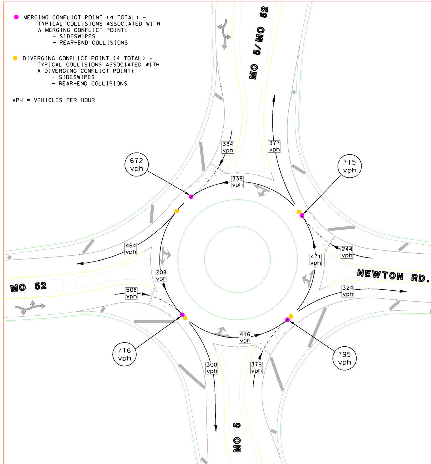
ROUNDBABOUT - 8 CONFLICT POINTS
