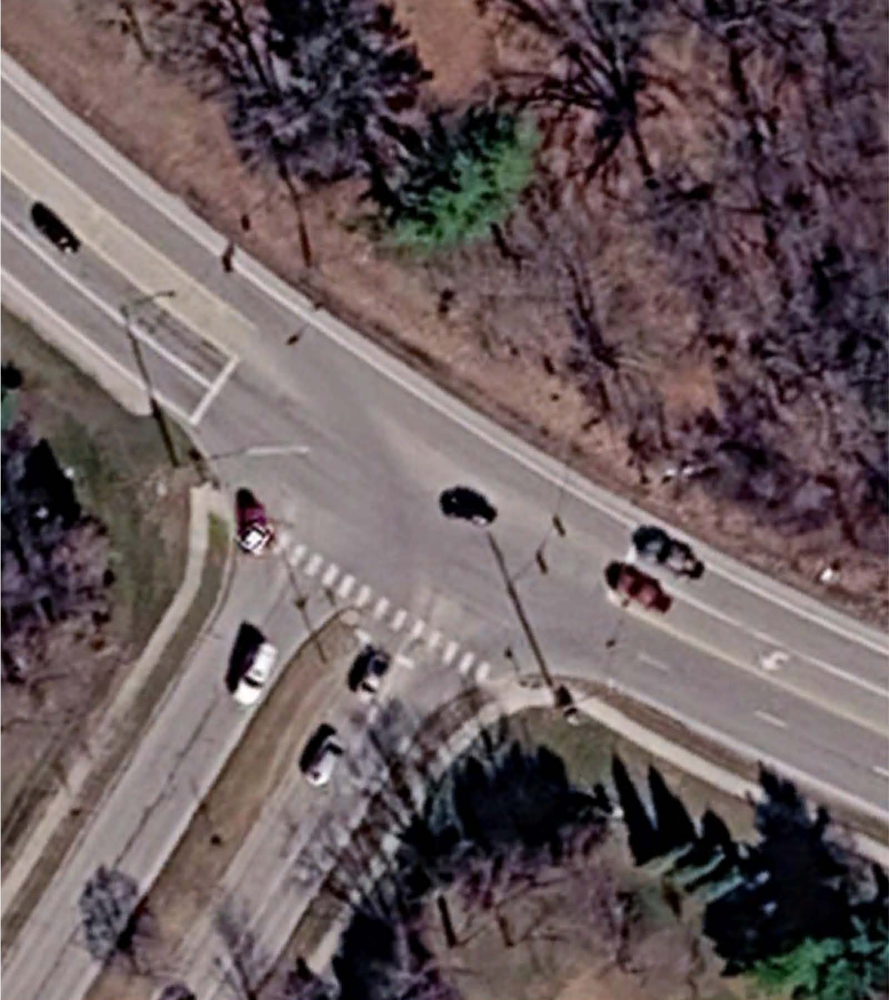
Current configuration at Flintlock Road and MO-291
