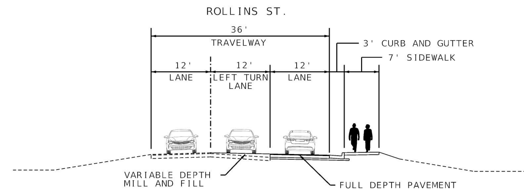
PROPOSED ROLLINS STREET TYPICAL SECTION
