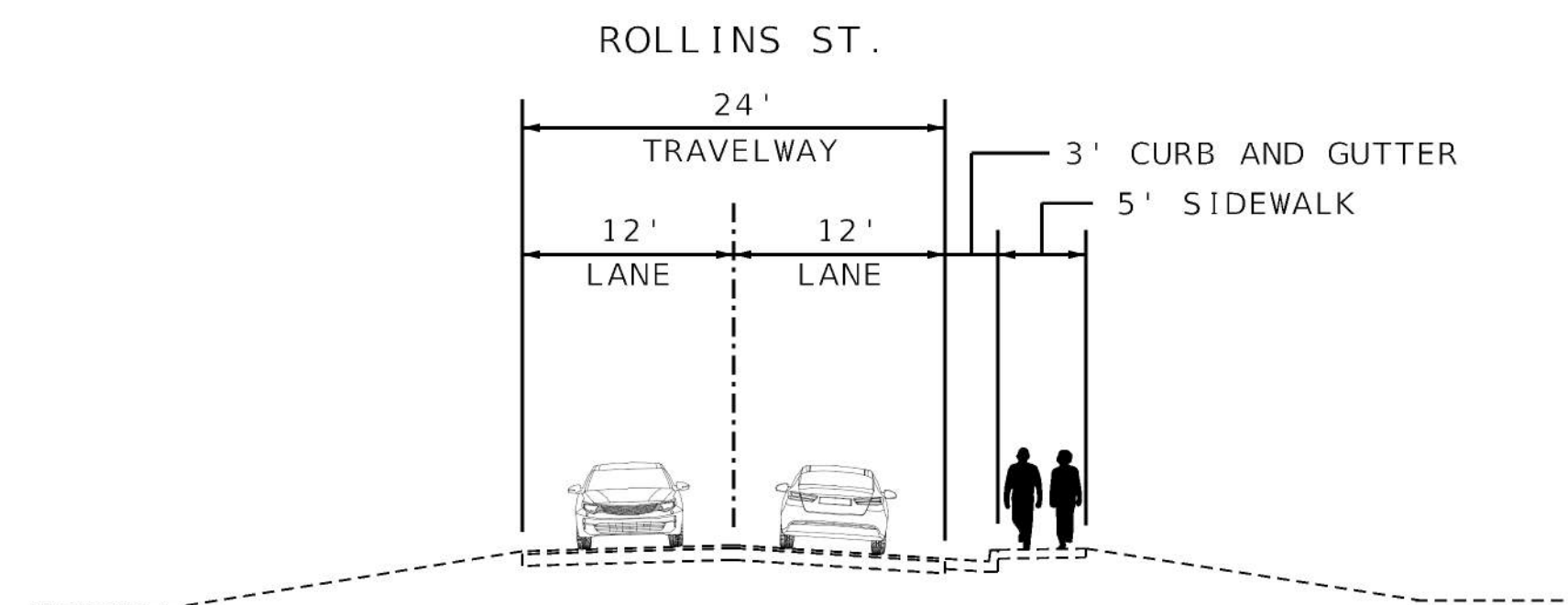
EXISTING ROLLINS STREET TYPICAL SECTION
