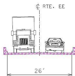
EXISTING BRIDGE TYPICAL SECTION
