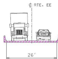
PROPOSED BRIDGE TYPICAL SECTION
