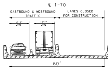
BRIDGE TYPICAL SECTION DURING CONSTRUCTION
