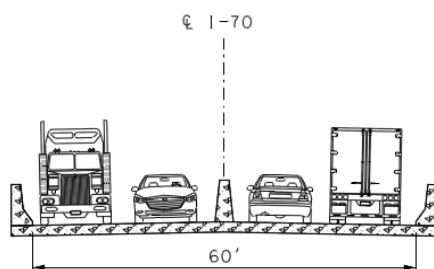
EXISTING BRIDGE TYPICAL SECTION
