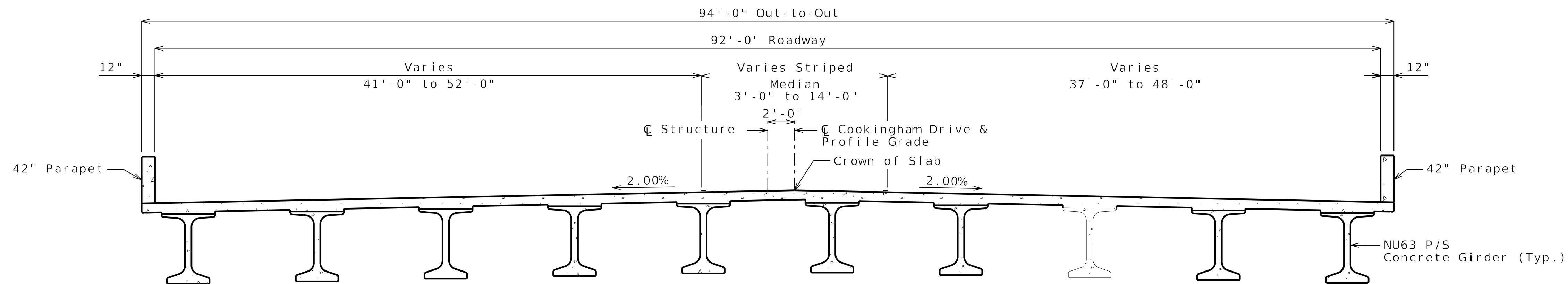
PROPOSED TYPICAL SECTION
