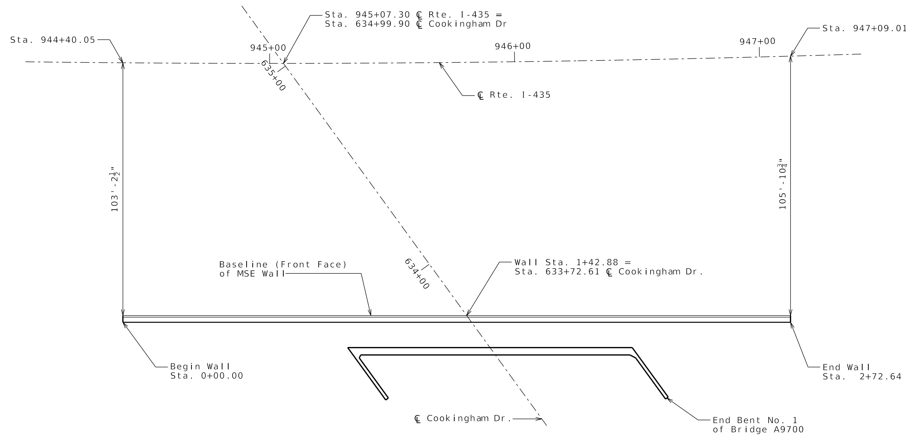
PLAN
