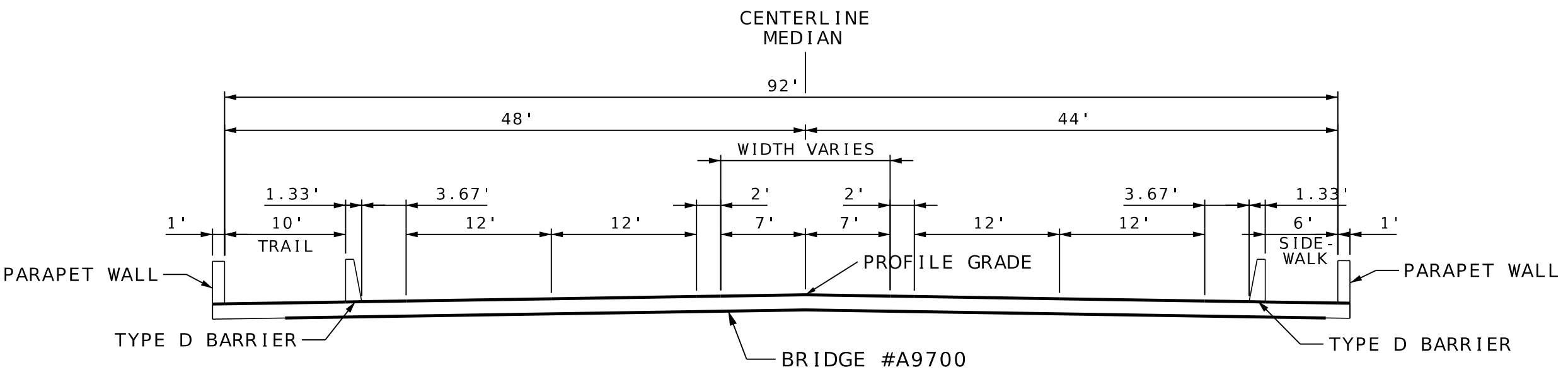
SECTION ON TANGENT TYPICAL SECTION BRIDGE FUTURE LAYOUT
