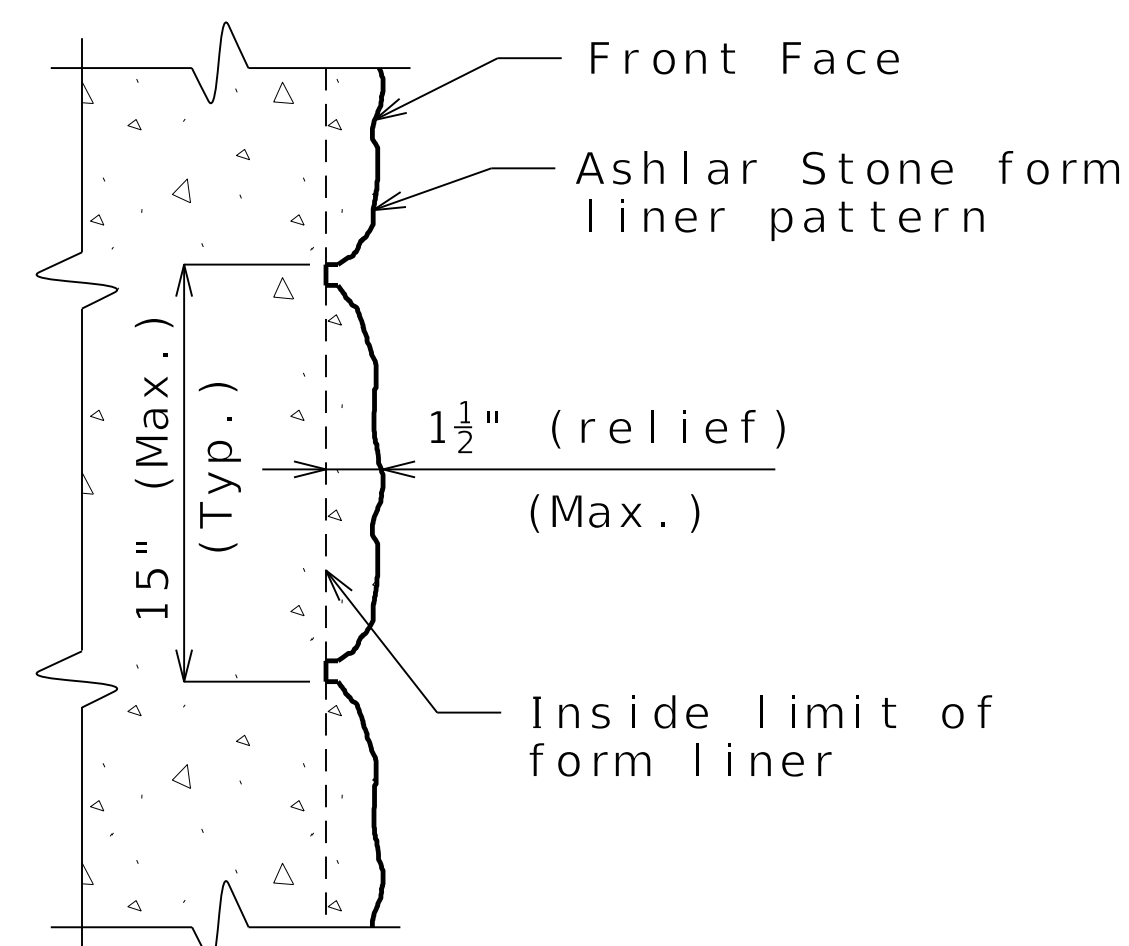
FORM LINER DETAIL (PRECAST MODULAR PANEL WALL)
