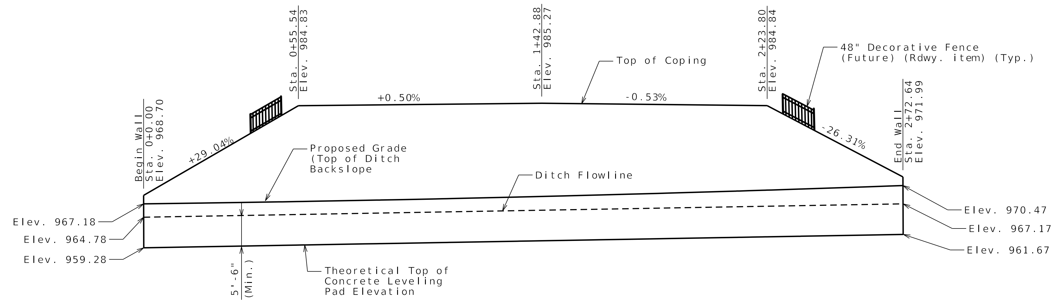
DEVELOPED ELEVATION
