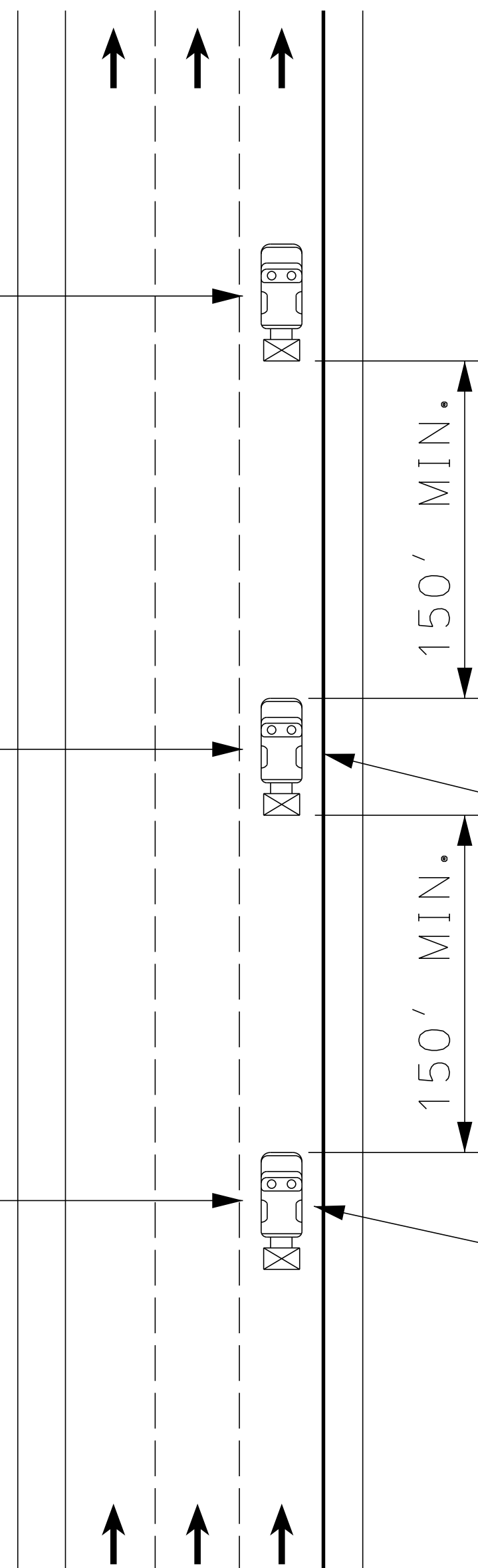
MULTI-LANE DIVIDED HIGHWAY
