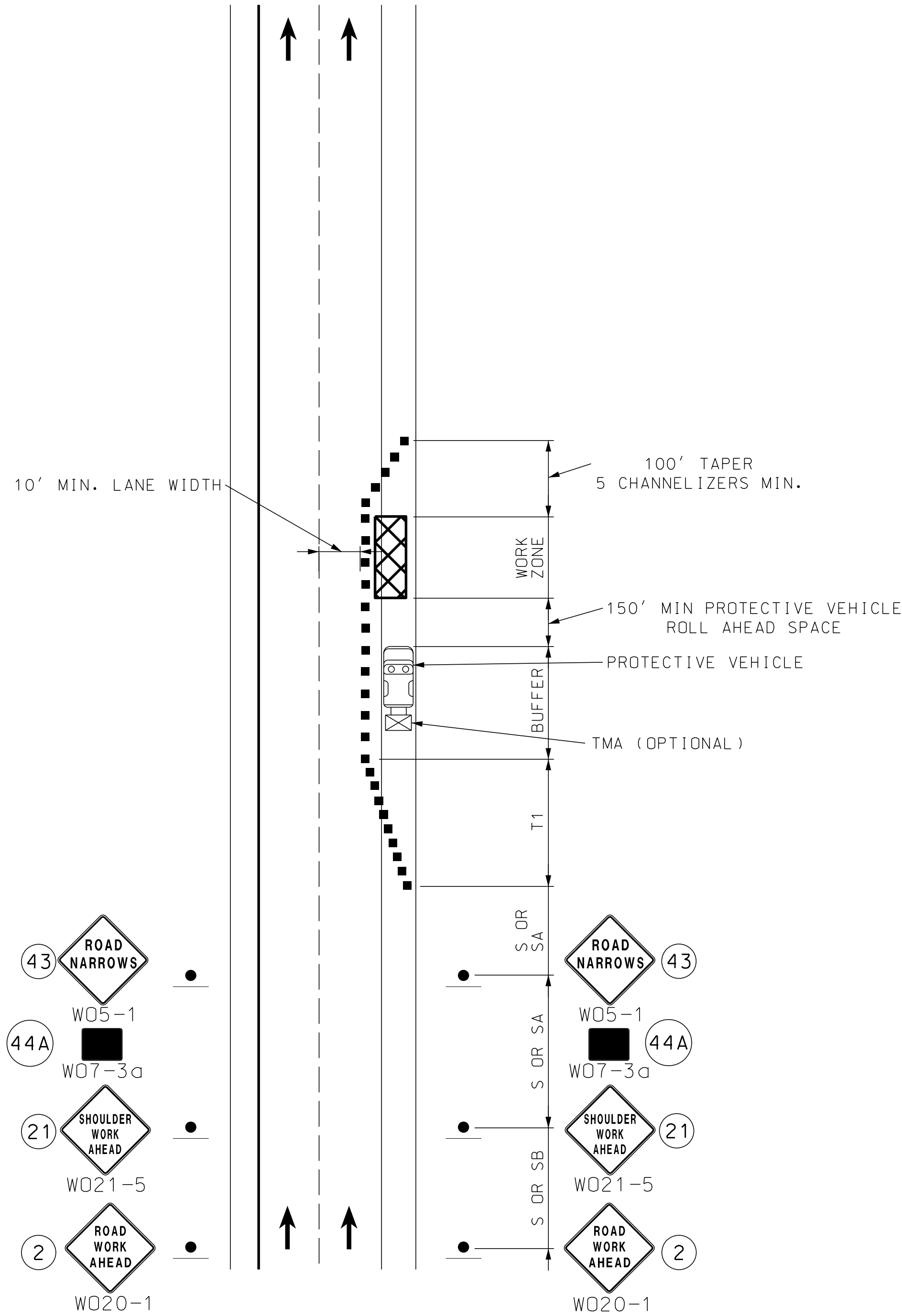
I-435 SHOULDER WORK WITH MINOR ENCROACHMENT ON DIVIDED AND UNDIVIDED HIGHWAYS
