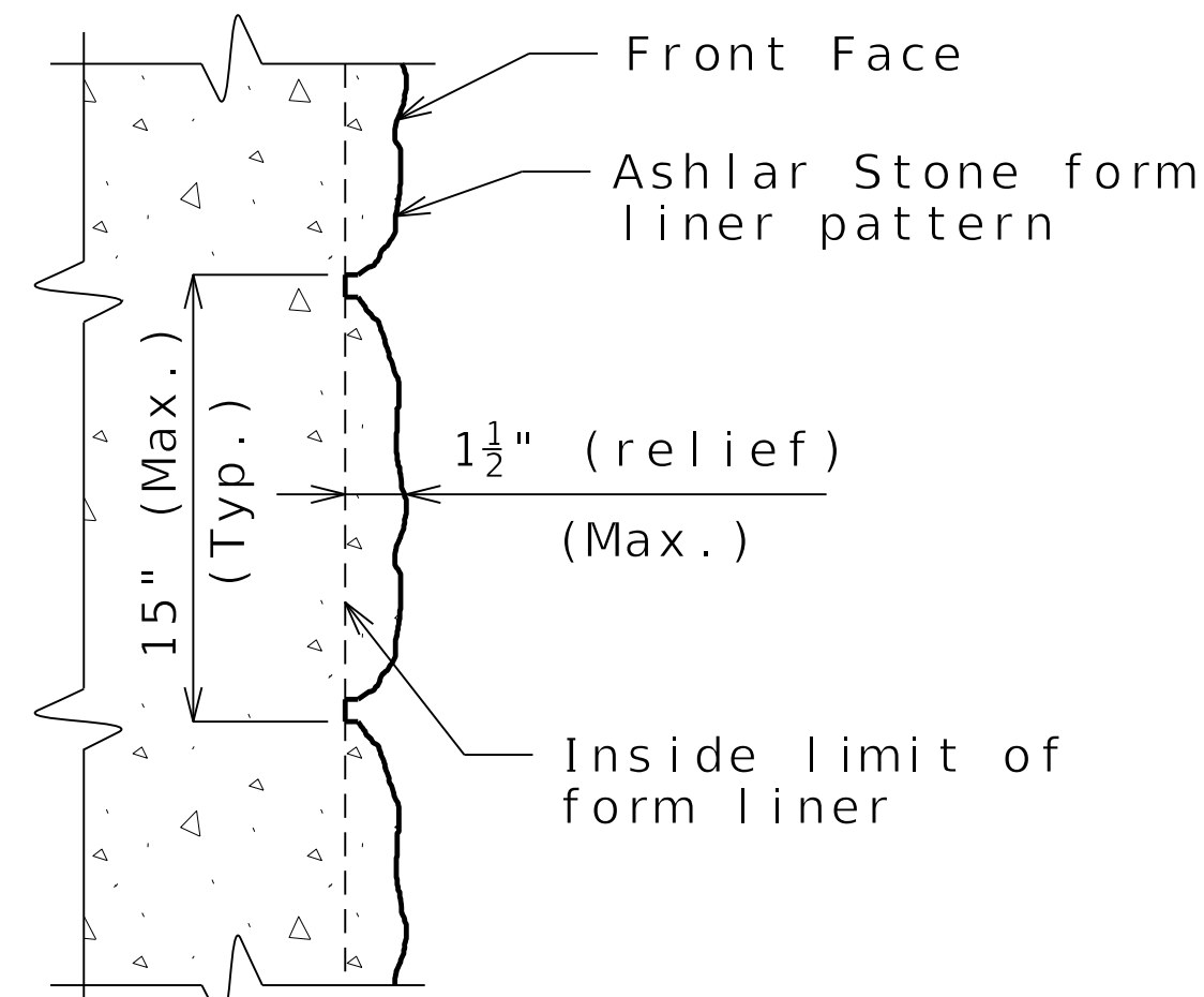
FORM LINER DETAIL (PRECAST MODULAR PANEL WALL)
