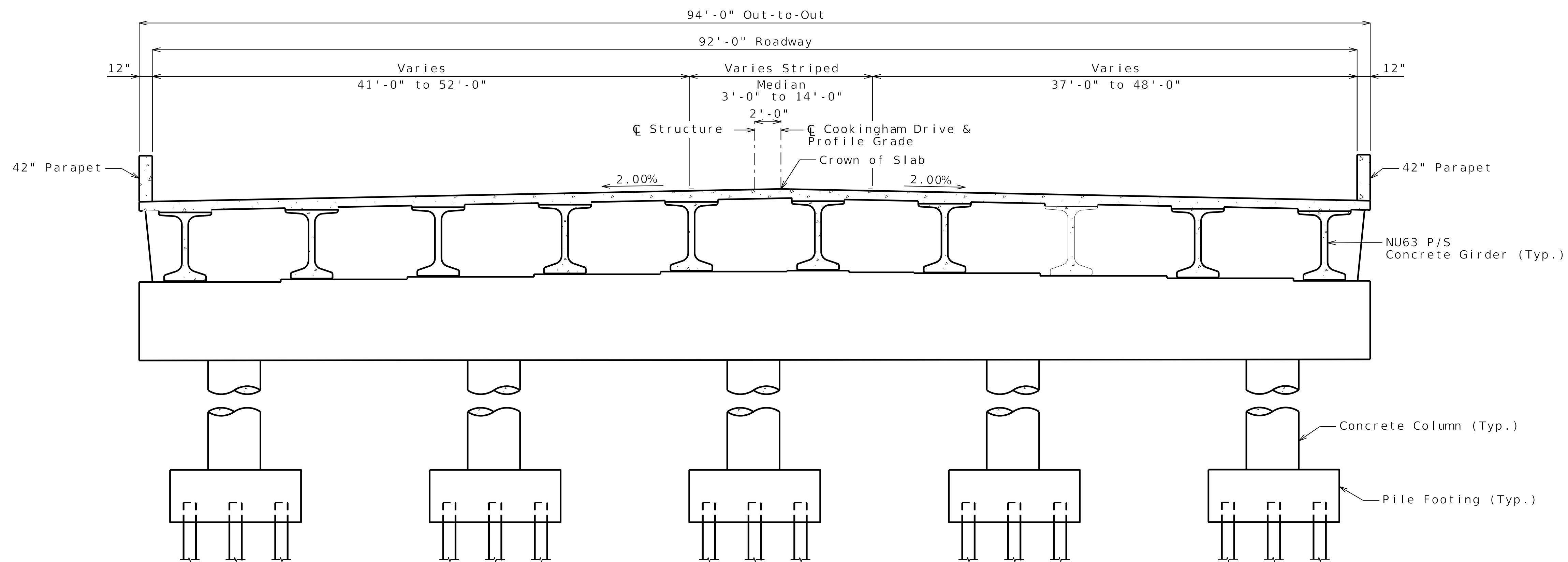
PROPOSED TYPICAL SECTION AT INTERMEDIATE BENT
