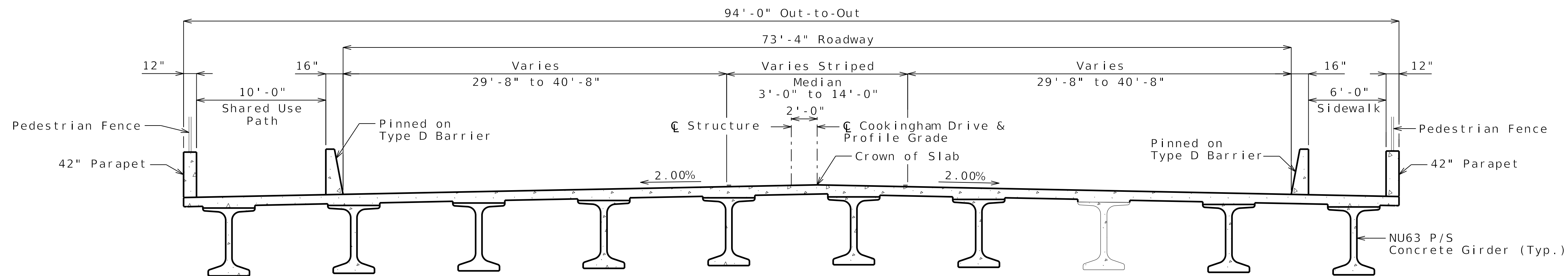
FUTURE TYPICAL SECTION
