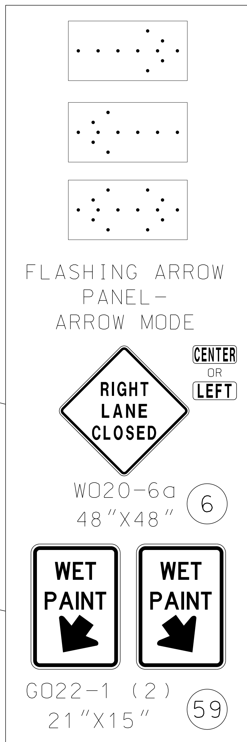
MULTI-LANE DIVIDED HIGHWAY
