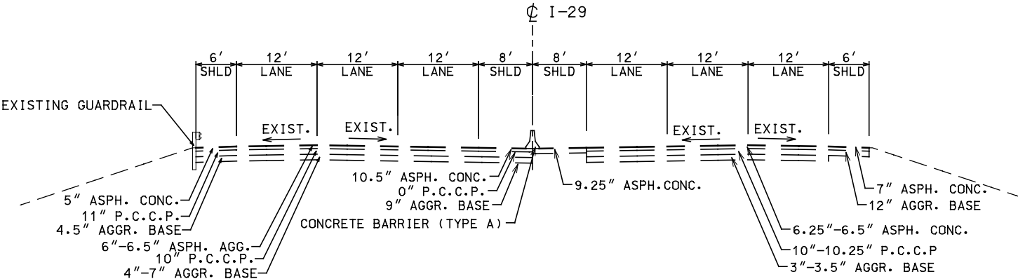
TYPICAL SECTION - I-29 NORTH OF 56TH ST. EXISTING
