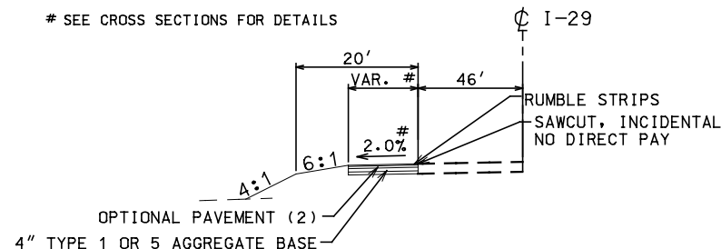
TYPICAL SECTION - I-29 STA. 897+00.00 TO 900+19.37
