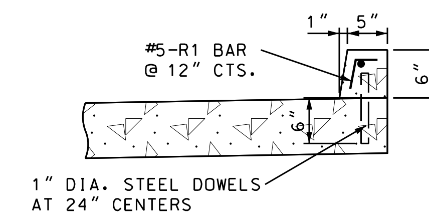
SECTION C-C
