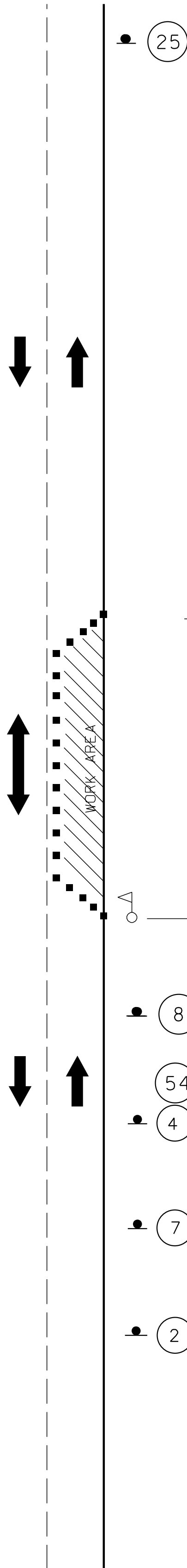
TA-10 LANE CLOSURE ON TWO-LANE ROAD USING FLAGGERS
