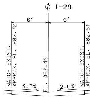
SEC. D-D 900+04.25 (I-29)
