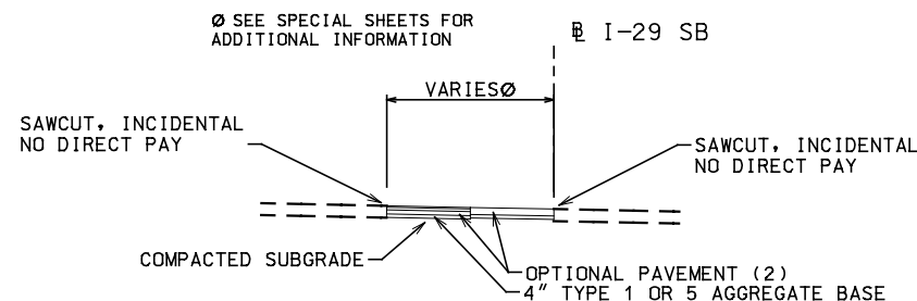
TYPICAL SECTION - I-29 STA. 904+65.07 TO 907+75.00 I-29 SB
