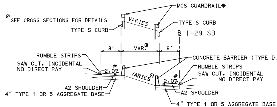
TYPICAL SECTION - I-29 STA. 904+65.07 TO 907+75.00 I-29 SB
