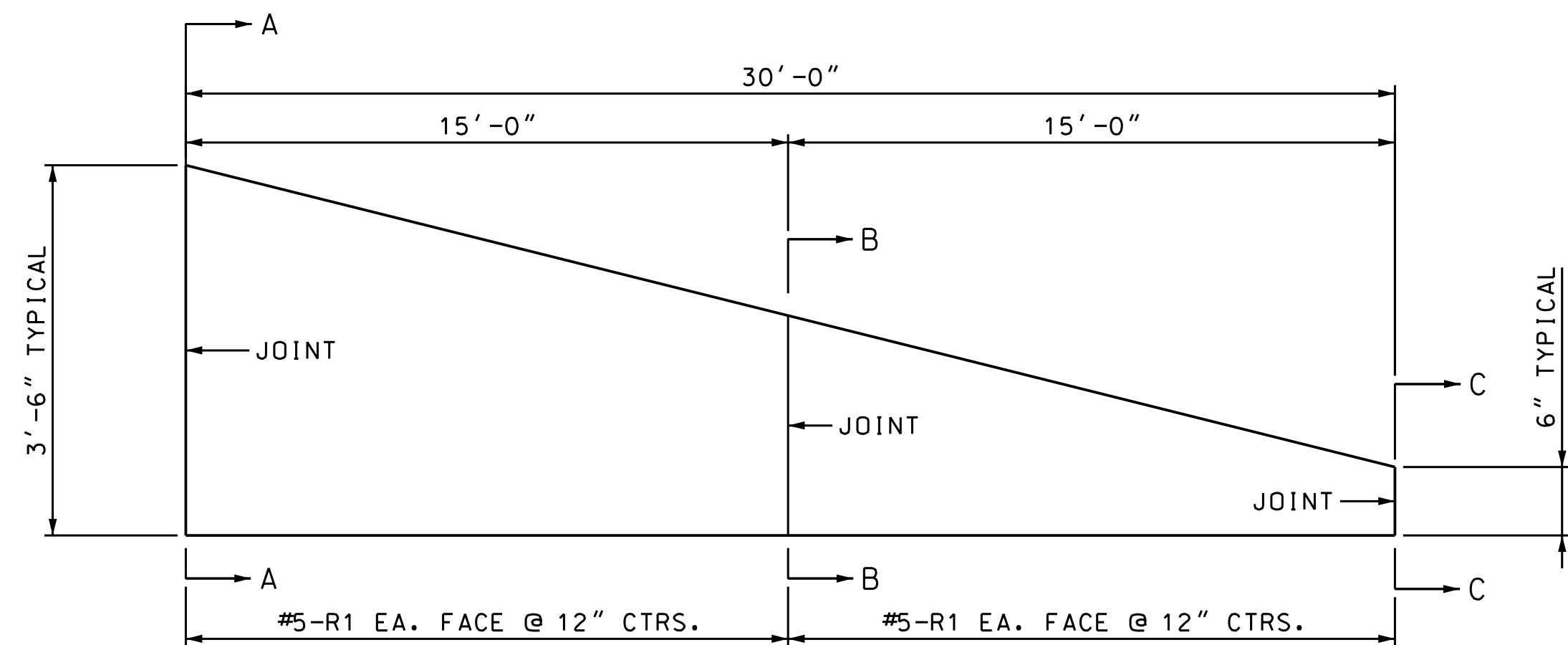
ELEVATION BARRIER HEIGHT TRANSITION
