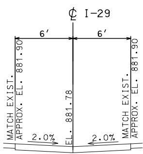
SEC. F-F 901+54.25 (I-29)
