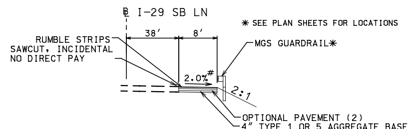
TYPICAL SECTION - I-29 SB LN STA. 904+65.07 TO 905+80.00
