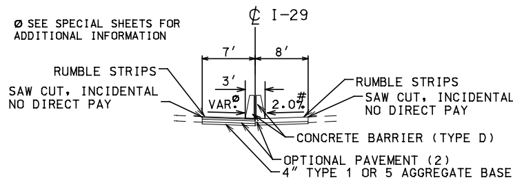
TYPICAL SECTION - I-29 STA. 902+95.25 TO 904+73.95 I-29
