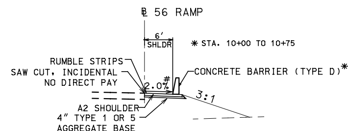
TYPICAL SECTION - 56TH RAMP STA. 10+00 TO 11+00
