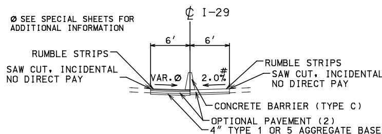
TYPICAL SECTION - I-29 STA. 896+50 TO 889+97.53 STA. 900+04.31 TO 901+54.75
