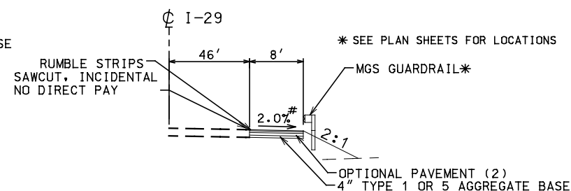
TYPICAL SECTION - I-29 STA. 897+20 TO 901+54.75 STA. 902+95.25 TO 904+73.95
