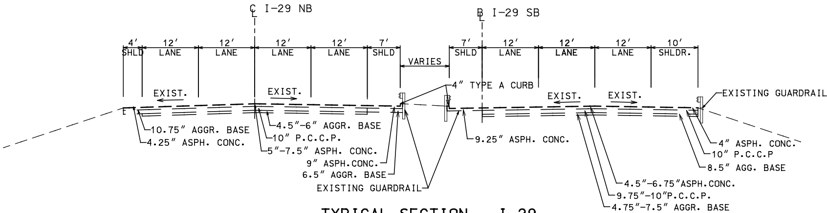
TYPICAL SECTION - I-29 SOUTH OF 56TH ST. EXISTING
