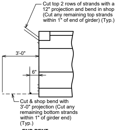
END BENT STRANDS AT GIRDER ENDS
