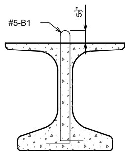
B1 BAR PERMISSIBLE ALTERNATE SHAPE
