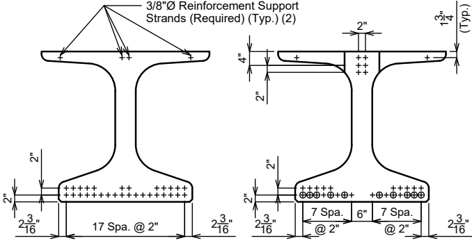
CL GIRDER STRAND ARRANGEMENT
