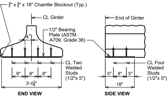
BEARING PLATE
