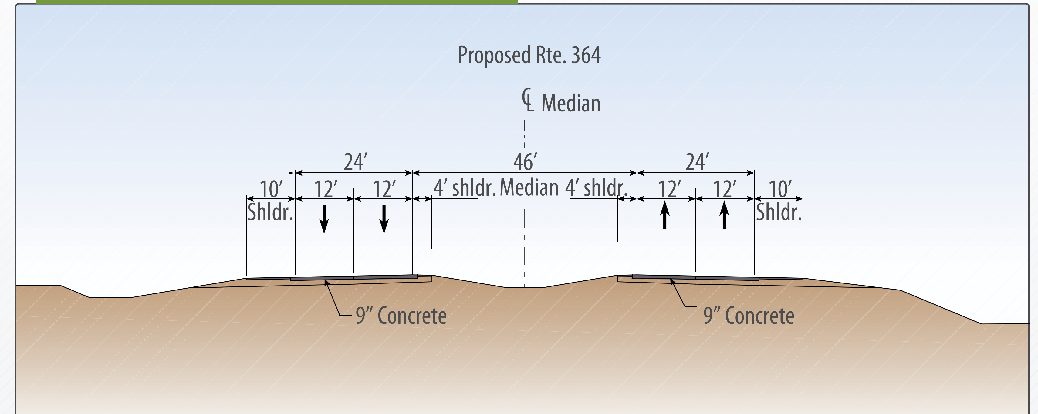
Route 364 Typical Section – Proposed 4-Lane Section
