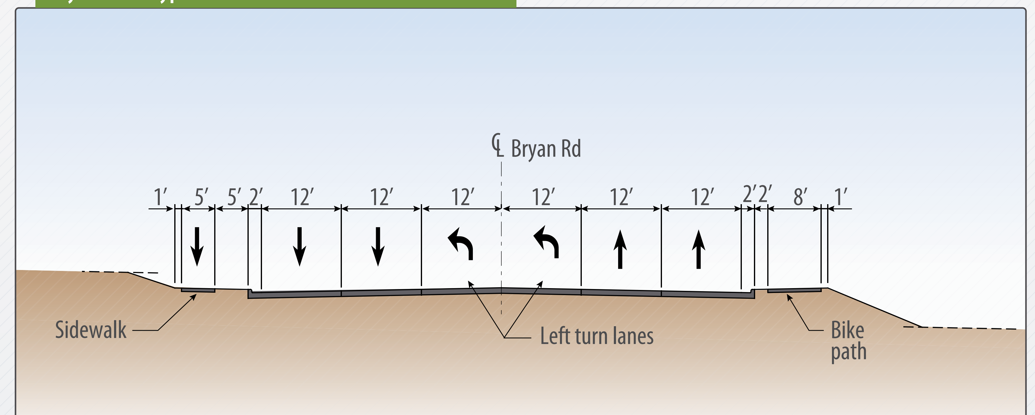
Bryan Road Typical Section
