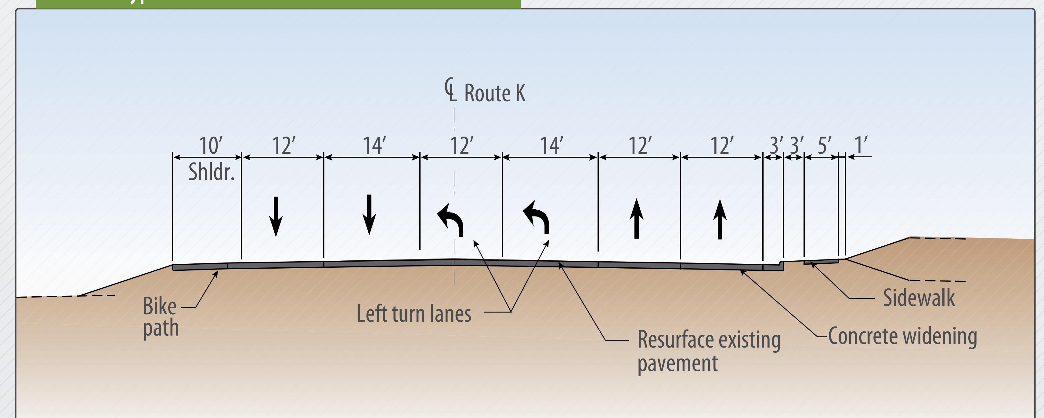
Route K Typical Section
