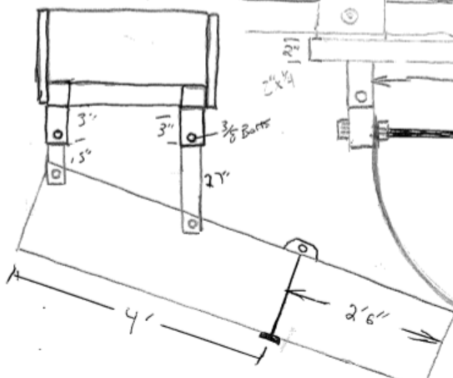
END VIEW
