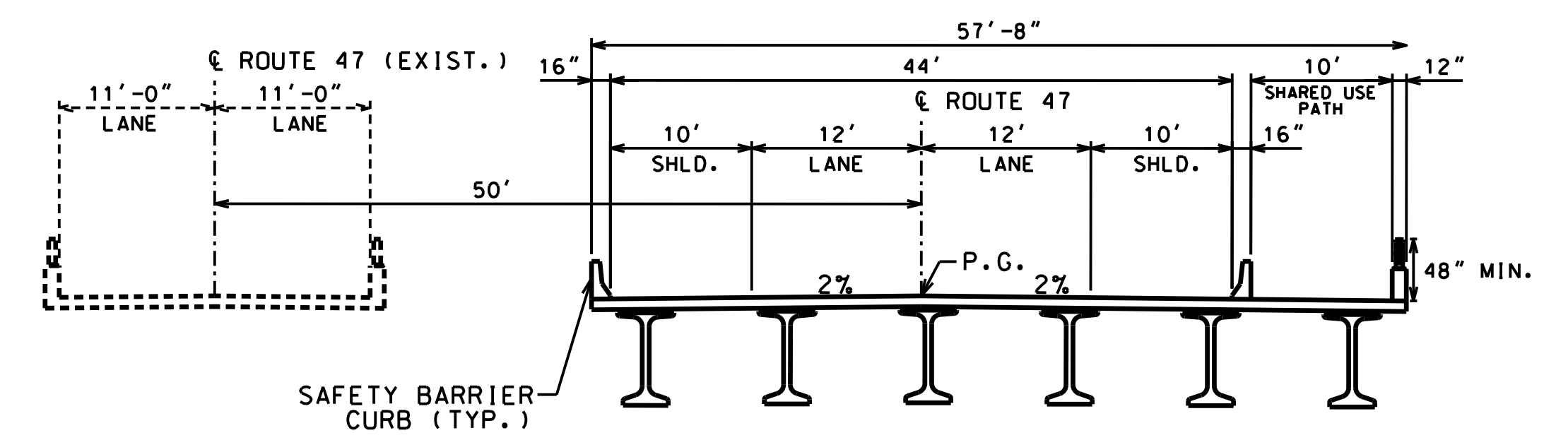
TYPICAL SECTION ON BRIDGE (LOOKING SOUTHBOUND)
