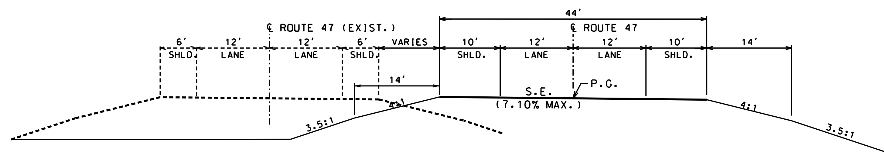
TYPICAL SECTION NORTH APPROACH (LOOKING SOUTHBOUND)
