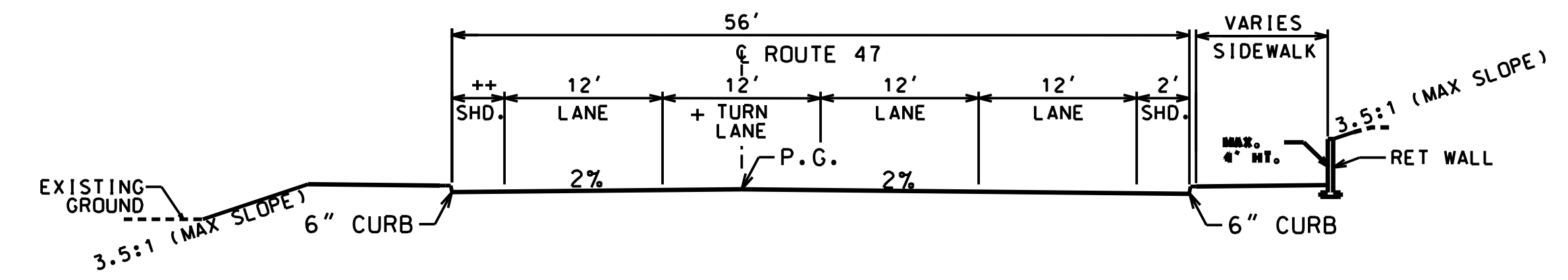
TYPICAL SECTION SOUTH APPROACH (LOOKING SOUTHBOUND)
