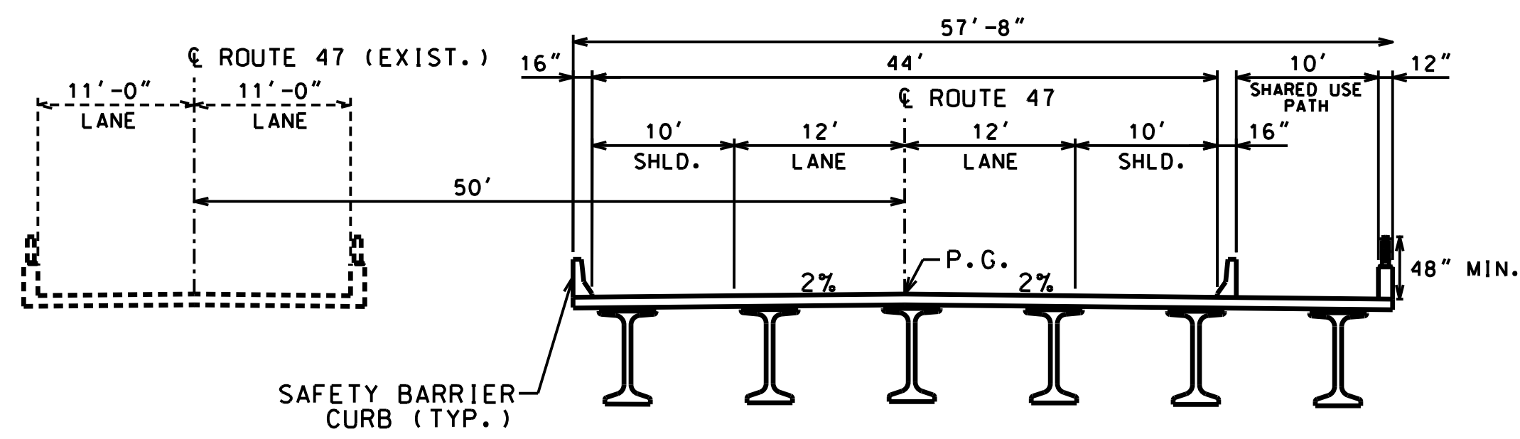
TYPICAL SECTION ON BRIDGE (LOOKING SOUTHBOUND)
