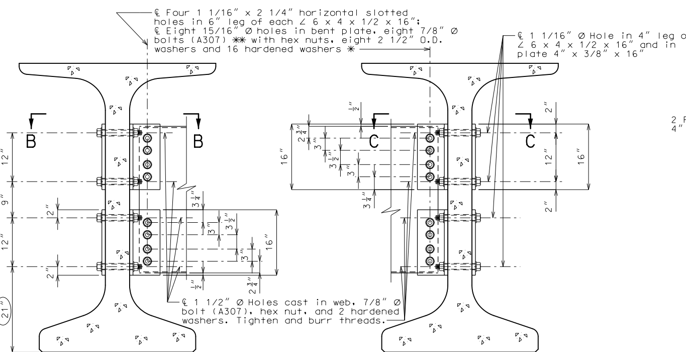
SECTION THRU INT. GIRDER AT DIAPHRAGM
