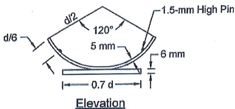
Figure 1 —Sutable Capping Device for Splitting Tensile Strength Test
