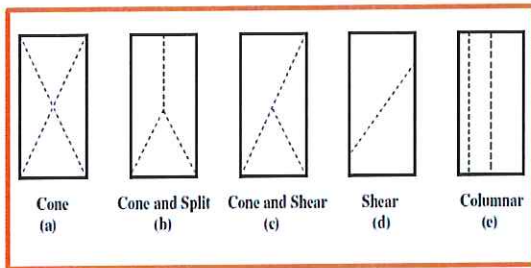
Figure 2: Types of Fracture Patterns
