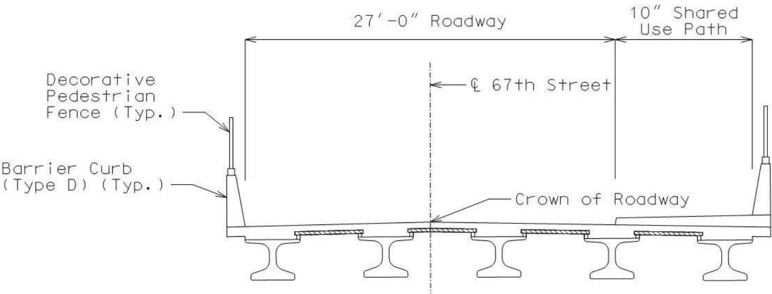
PROPOSED BRIDGE SECTION
