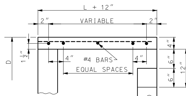
SECTION N-N
