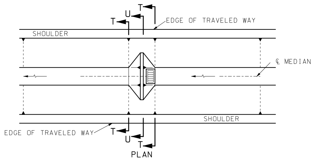
PLAN
