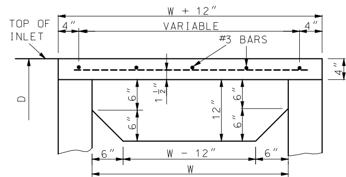
SECTION M-M
