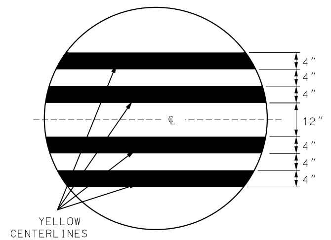
DETAIL B
