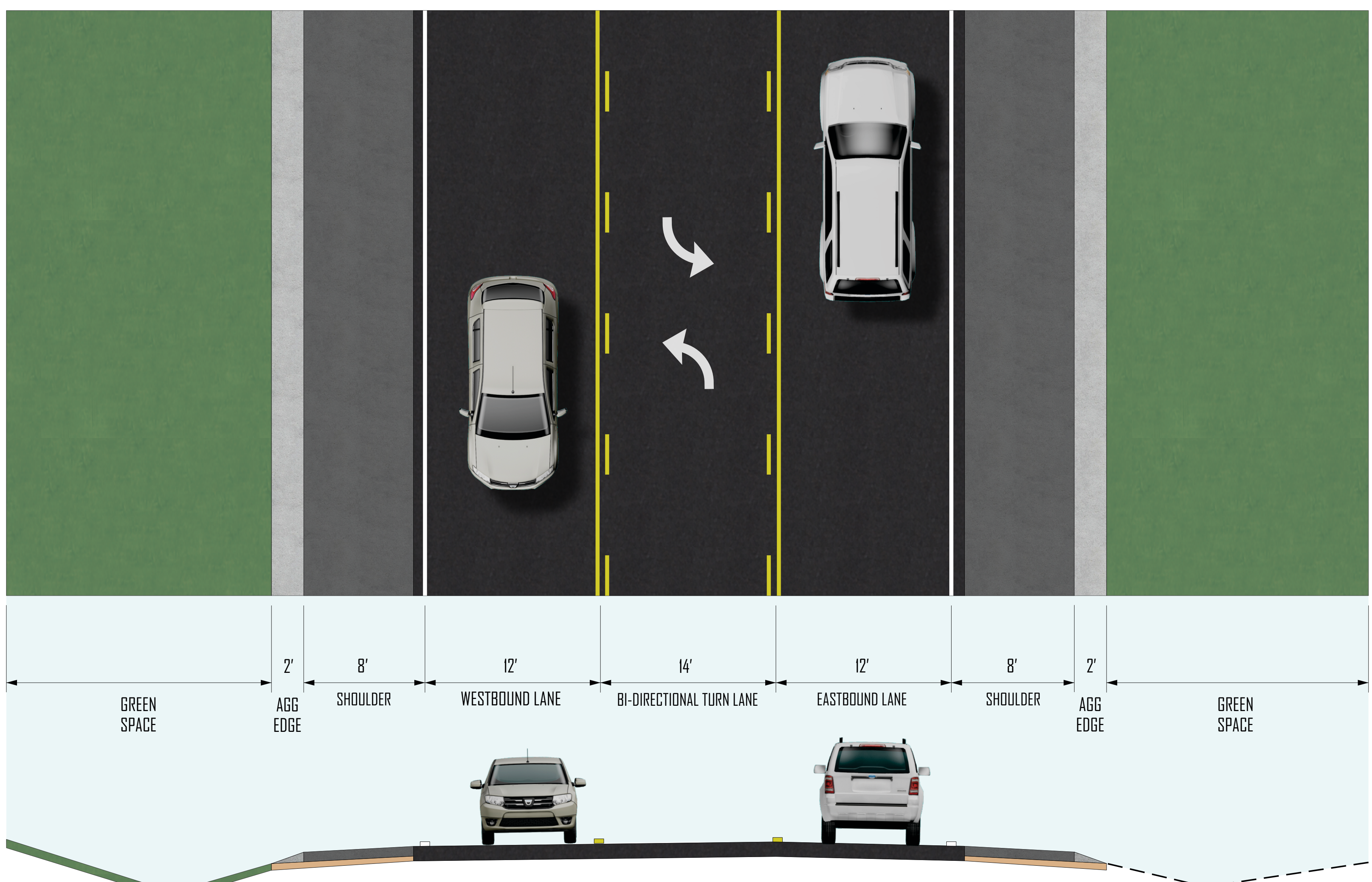
THREE LANE SECTION (BENNINGTON DRIVE TO ROUTE H)
