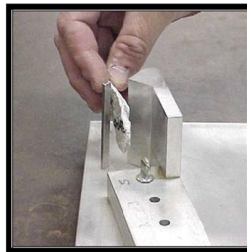
Figure 2 Checking Flatness
